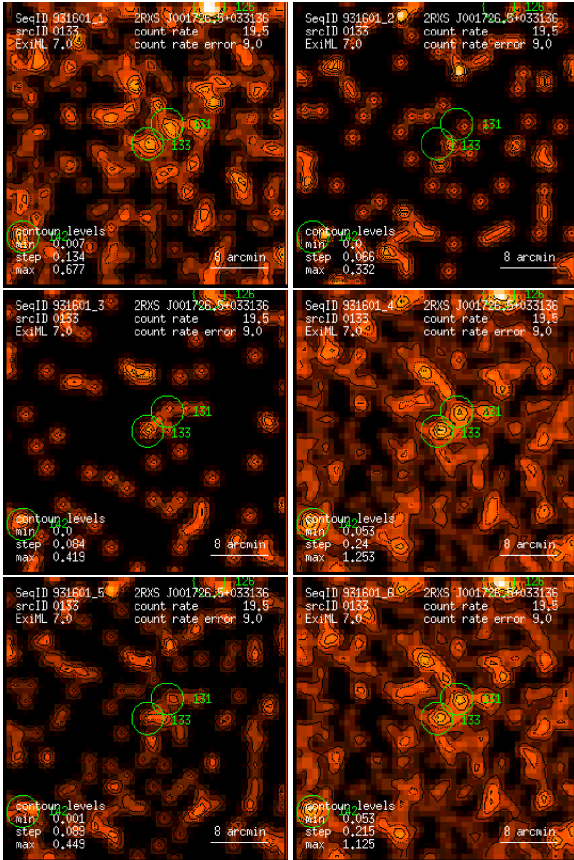
Figure 133: RASS 931601: detection 0133: band rate images, Gaussian filter: (1) PSPC channels 11 – 41, (2) 52 – 90, (3) 91 – 201, (4) 11 – 235, (5) 52 – 201, (6) 11 – 201. Broad band rates in counts/ks. Band rate contour levels in counts/ks/arcmin 2 .
