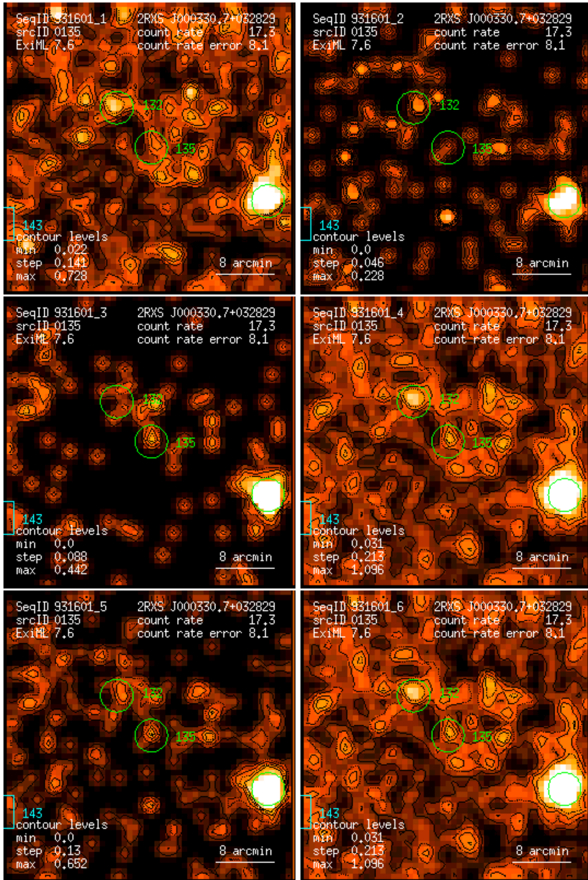
Figure 135: RASS 931601: detection 0135: band rate images, Gaussian filter: (1) PSPC channels 11 – 41, (2) 52 – 90, (3) 91 – 201, (4) 11 – 235, (5) 52 – 201, (6) 11 – 201. Broad band rates in counts/ks. Band rate contour levels in counts/ks/arcmin 2 .
