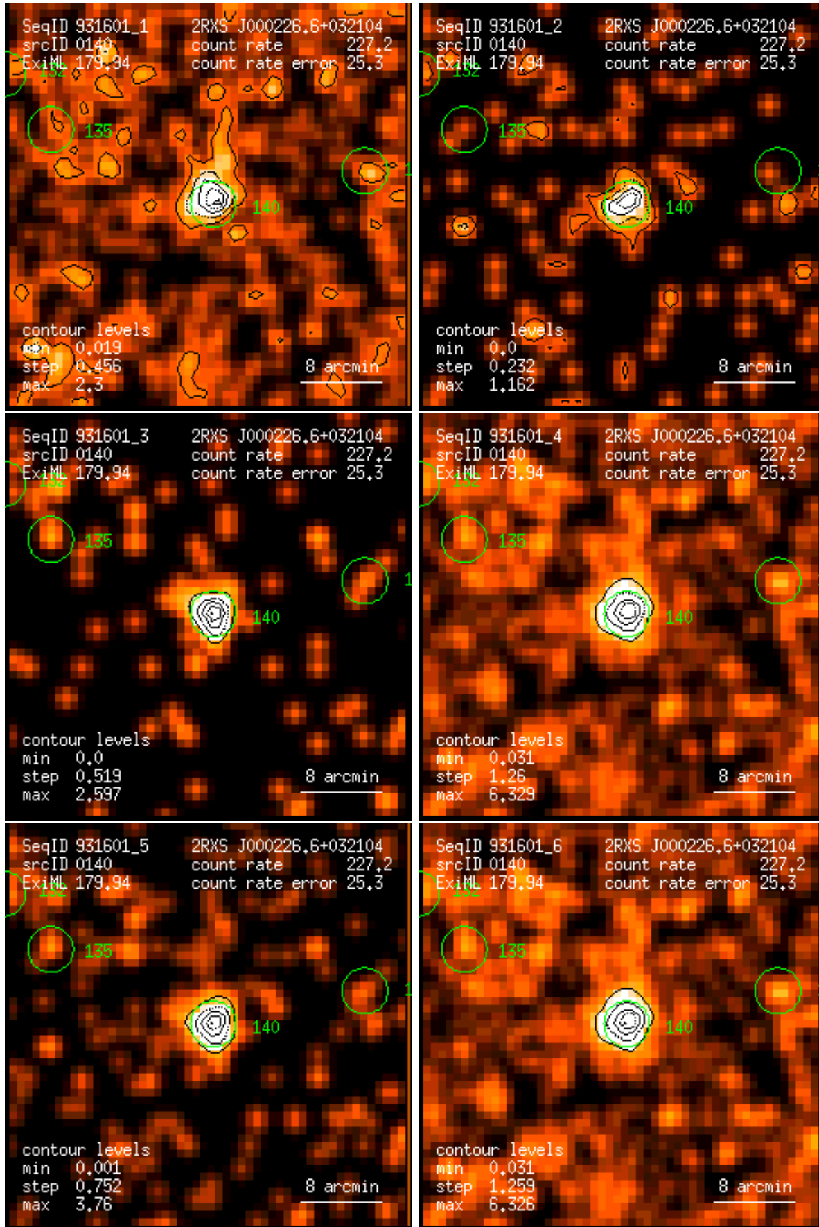
Figure 140: RASS 931601: detection 0140: band rate images, Gaussian filter: (1) PSPC channels 11 – 41, (2) 52 – 90, (3) 91 – 201, (4) 11 – 235, (5) 52 – 201, (6) 11 – 201. Broad band rates in counts/ks. Band rate contour levels in counts/ks/arcmin 2 .
