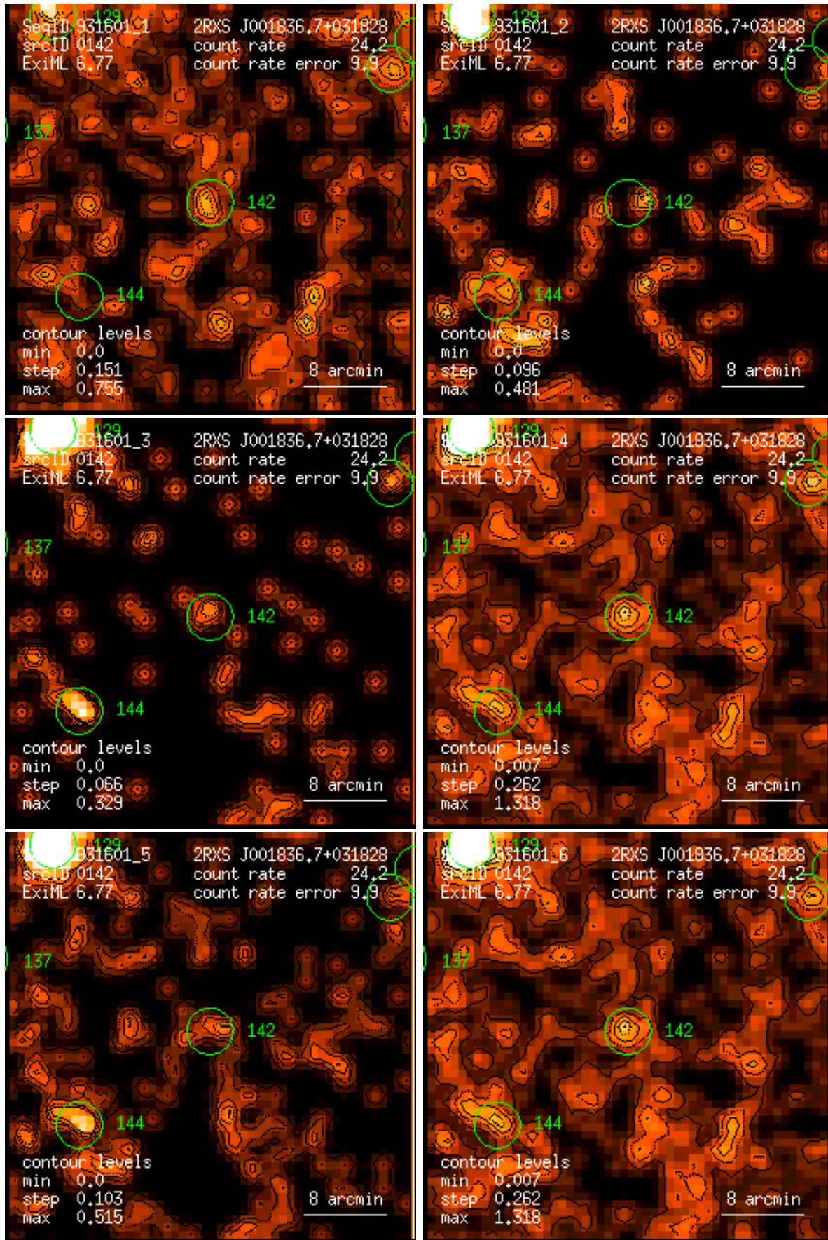
Figure 142: RASS 931601: detection 0142: band rate images, Gaussian filter: (1) PSPC channels 11 – 41, (2) 52 – 90, (3) 91 – 201, (4) 11 – 235, (5) 52 – 201, (6) 11 – 201. Broad band rates in counts/ks. Band rate contour levels in counts/ks/arcmin 2 .
