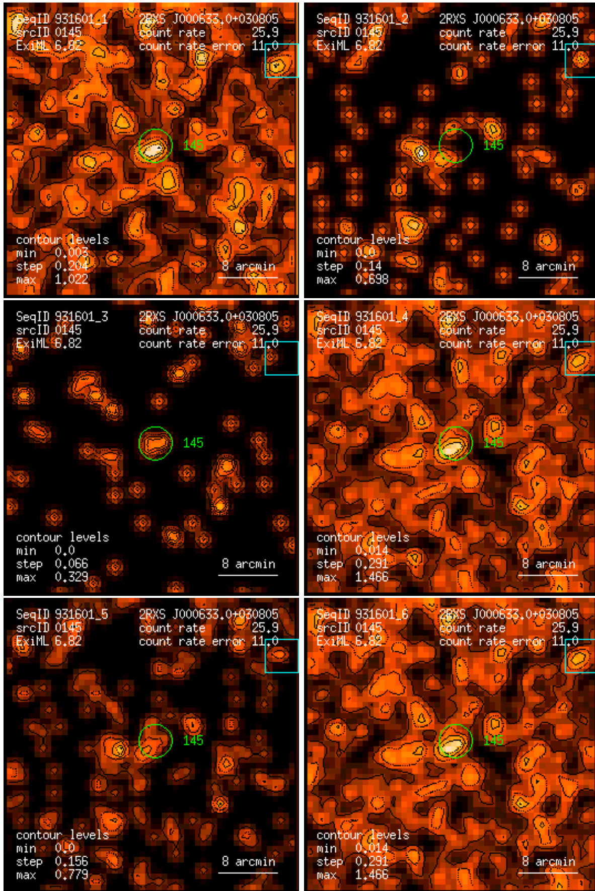
Figure 145: RASS 931601: detection 0145: band rate images, Gaussian filter: (1) PSPC channels 11 – 41, (2) 52 – 90, (3) 91 – 201, (4) 11 – 235, (5) 52 – 201, (6) 11 – 201. Broad band rates in counts/ks. Band rate contour levels in counts/ks/arcmin 2 .
