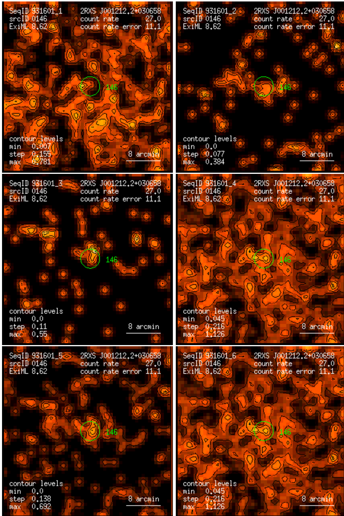
Figure 146: RASS 931601: detection 0146: band rate images, Gaussian filter: (1) PSPC channels 11 – 41, (2) 52 – 90, (3) 91 – 201, (4) 11 – 235, (5) 52 – 201, (6) 11 – 201. Broad band rates in counts/ks. Band rate contour levels in counts/ks/arcmin 2 .
