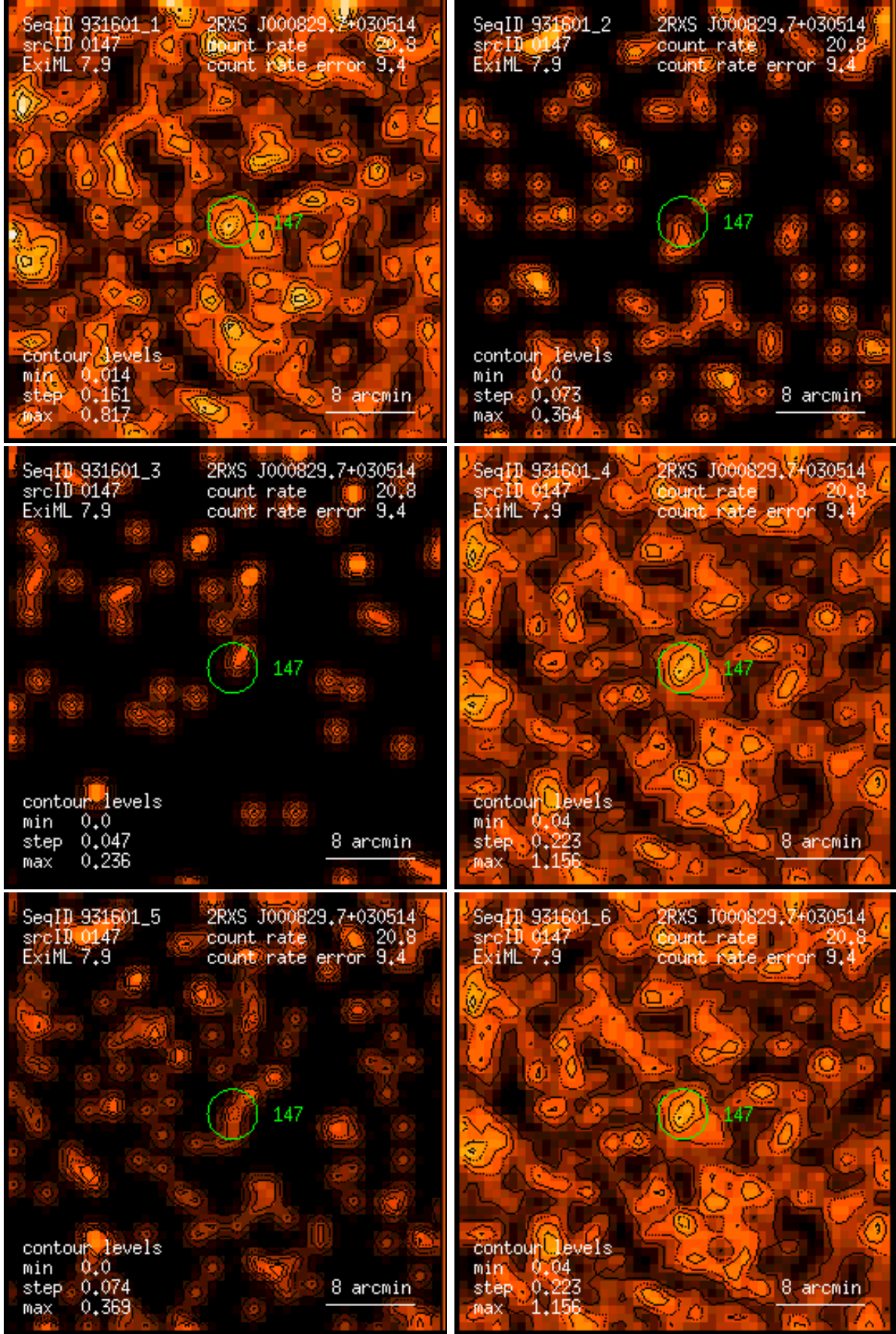
Figure 147: RASS 931601: detection 0147: band rate images, Gaussian filter: (1) PSPC channels 11 – 41, (2) 52 – 90, (3) 91 – 201, (4) 11 – 235, (5) 52 – 201, (6) 11 – 201. Broad band rates in counts/ks. Band rate contour levels in counts/ks/arcmin 2 .
