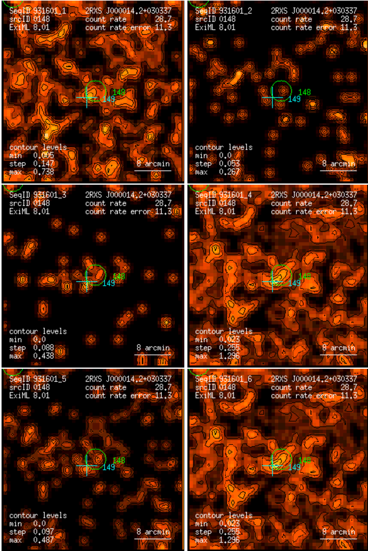
Figure 148: RASS 931601: detection 0148: band rate images, Gaussian filter: (1) PSPC channels 11 – 41, (2) 52 – 90, (3) 91 – 201, (4) 11 – 235, (5) 52 – 201, (6) 11 – 201. Broad band rates in counts/ks. Band rate contour levels in counts/ks/arcmin 2 .
