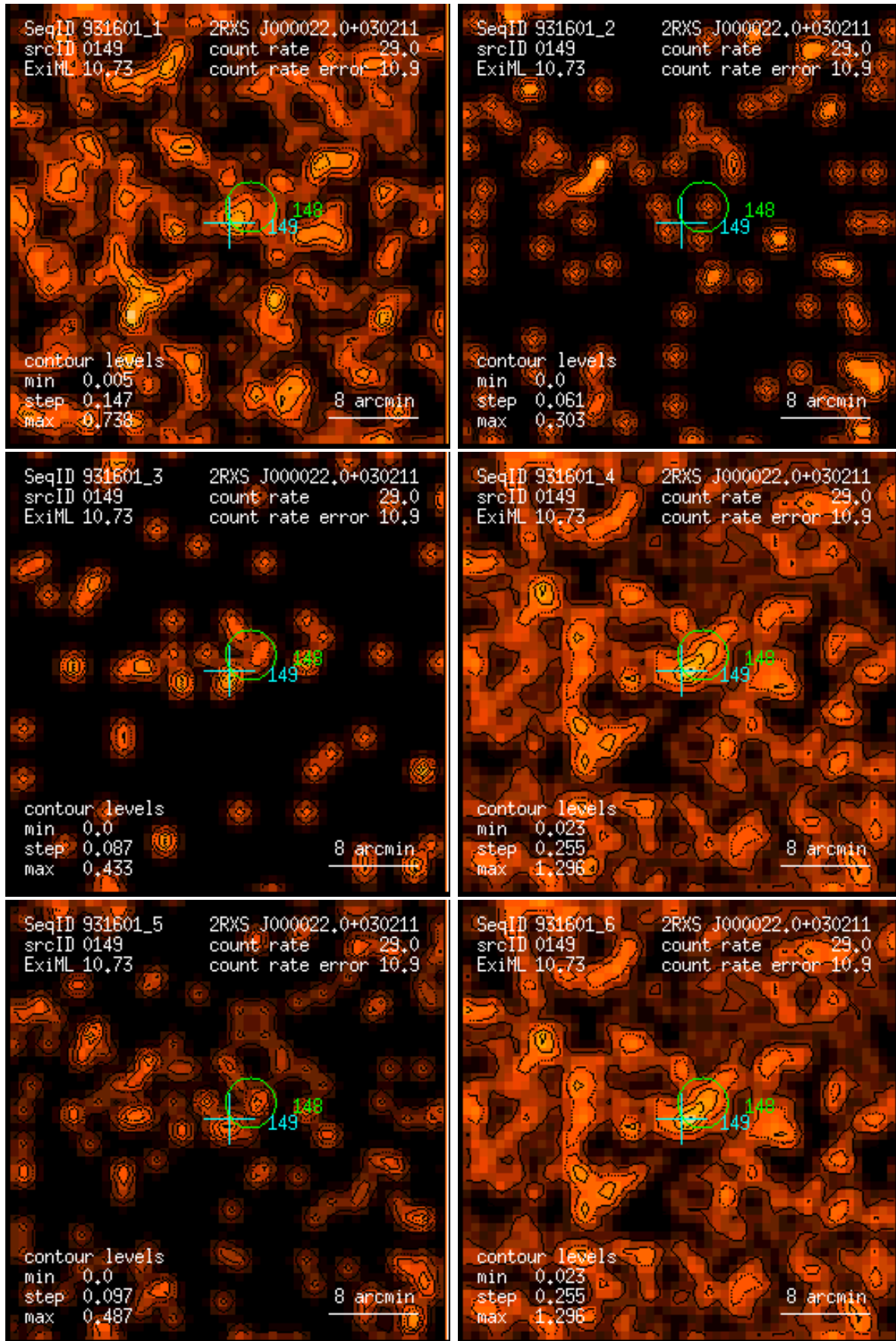
Figure 149: RASS 931601: detection 0149: band rate images, Gaussian filter: (1) PSPC channels 11 – 41, (2) 52 – 90, (3) 91 – 201, (4) 11 – 235, (5) 52 – 201, (6) 11 – 201. Broad band rates in counts/ks. Band rate contour levels in counts/ks/arcmin 2 .
