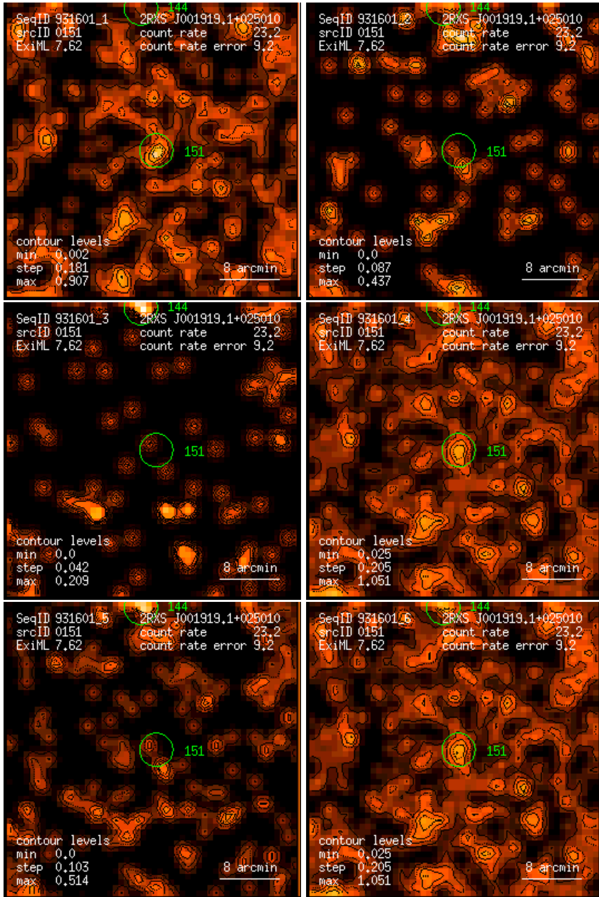
Figure 151: RASS 931601: detection 0151: band rate images, Gaussian filter: (1) PSPC channels 11 – 41, (2) 52 – 90, (3) 91 – 201, (4) 11 – 235, (5) 52 – 201, (6) 11 – 201. Broad band rates in counts/ks. Band rate contour levels in counts/ks/arcmin 2 .
