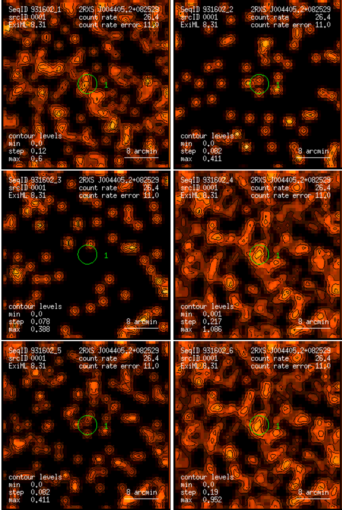
Figure 1: RASS 931602: detection 0001: band rate images, Gaussian filter: (1) PSPC channels 11 – 41, (2) 52 – 90, (3) 91 – 201, (4) 11 – 235, (5) 52 – 201, (6) 11 – 201. Broad band rates in counts/ks. Band rate contour levels in counts/ks/arcmin 2 .
