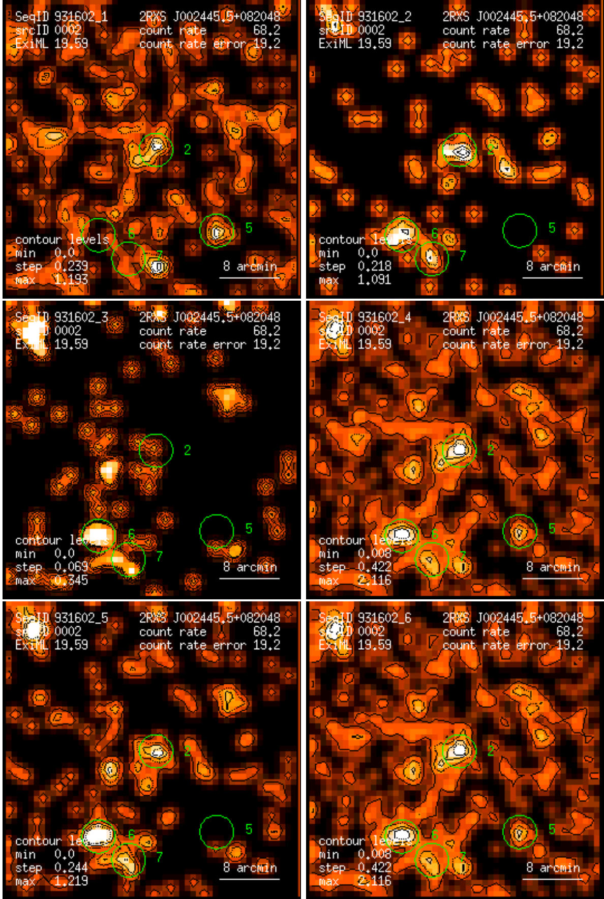
Figure 2: RASS 931602: detection 0002: band rate images, Gaussian filter: (1) PSPC channels 11 – 41, (2) 52 – 90, (3) 91 – 201, (4) 11 – 235, (5) 52 – 201, (6) 11 – 201. Broad band rates in counts/ks. Band rate contour levels in counts/ks/arcmin 2 .
