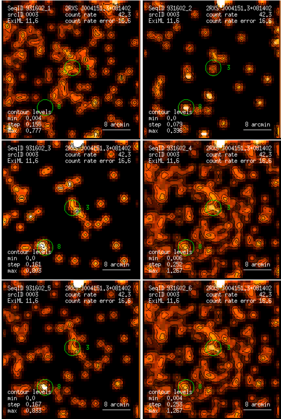
Figure 3: RASS 931602: detection 0003: band rate images, Gaussian filter: (1) PSPC channels 11 – 41, (2) 52 – 90, (3) 91 – 201, (4) 11 – 235, (5) 52 – 201, (6) 11 – 201. Broad band rates in counts/ks. Band rate contour levels in counts/ks/arcmin 2 .
