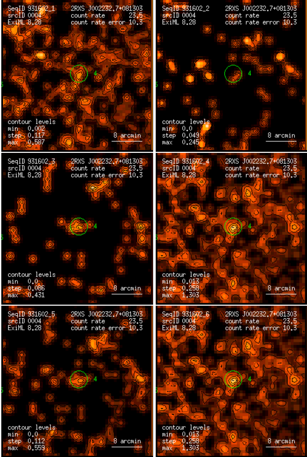
Figure 4: RASS 931602: detection 0004: band rate images, Gaussian filter: (1) PSPC channels 11 – 41, (2) 52 – 90, (3) 91 – 201, (4) 11 – 235, (5) 52 – 201, (6) 11 – 201. Broad band rates in counts/ks. Band rate contour levels in counts/ks/arcmin 2 .
