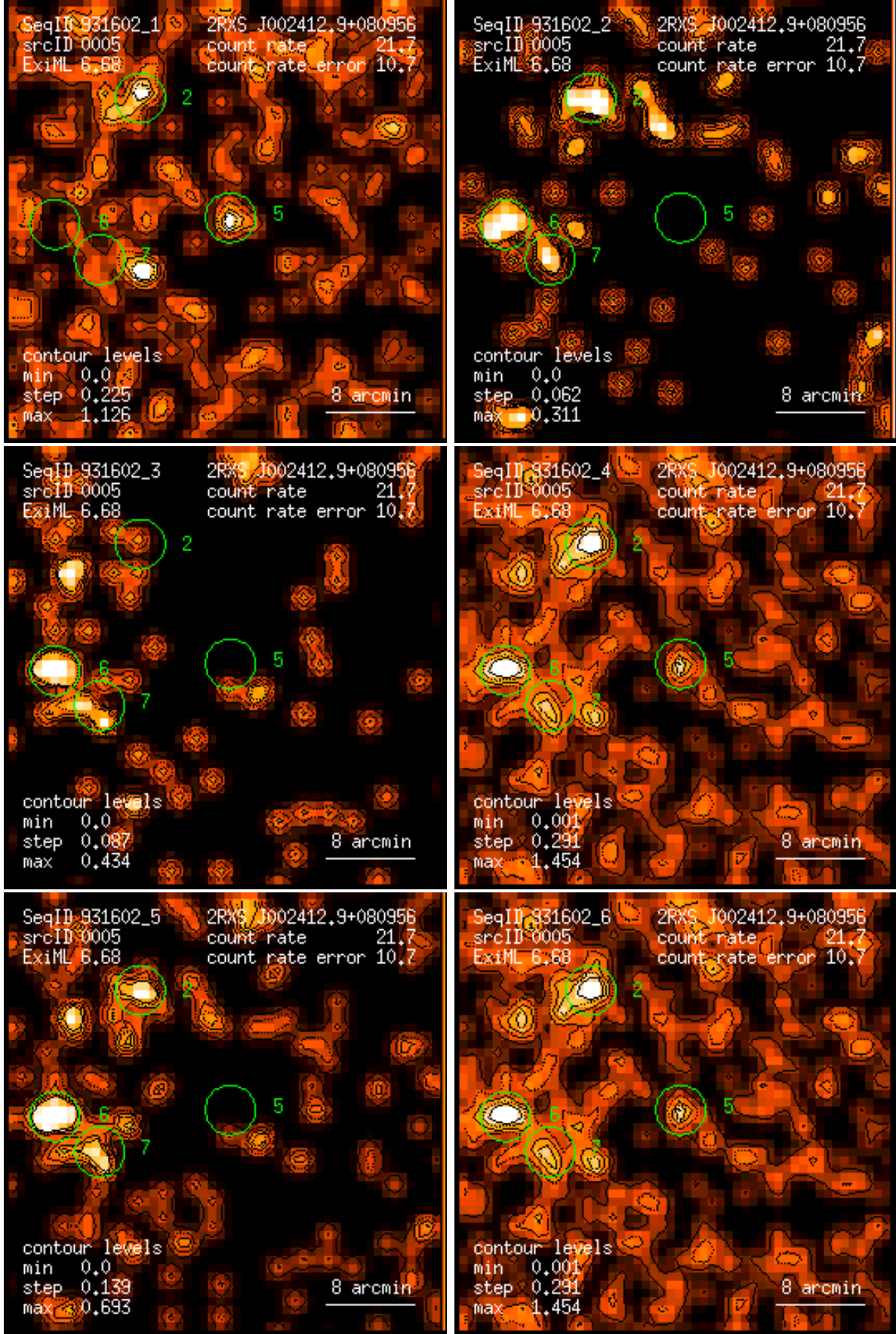
Figure 5: RASS 931602: detection 0005: band rate images, Gaussian filter: (1) PSPC channels 11 – 41, (2) 52 – 90, (3) 91 – 201, (4) 11 – 235, (5) 52 – 201, (6) 11 – 201. Broad band rates in counts/ks. Band rate contour levels in counts/ks/arcmin 2 .
