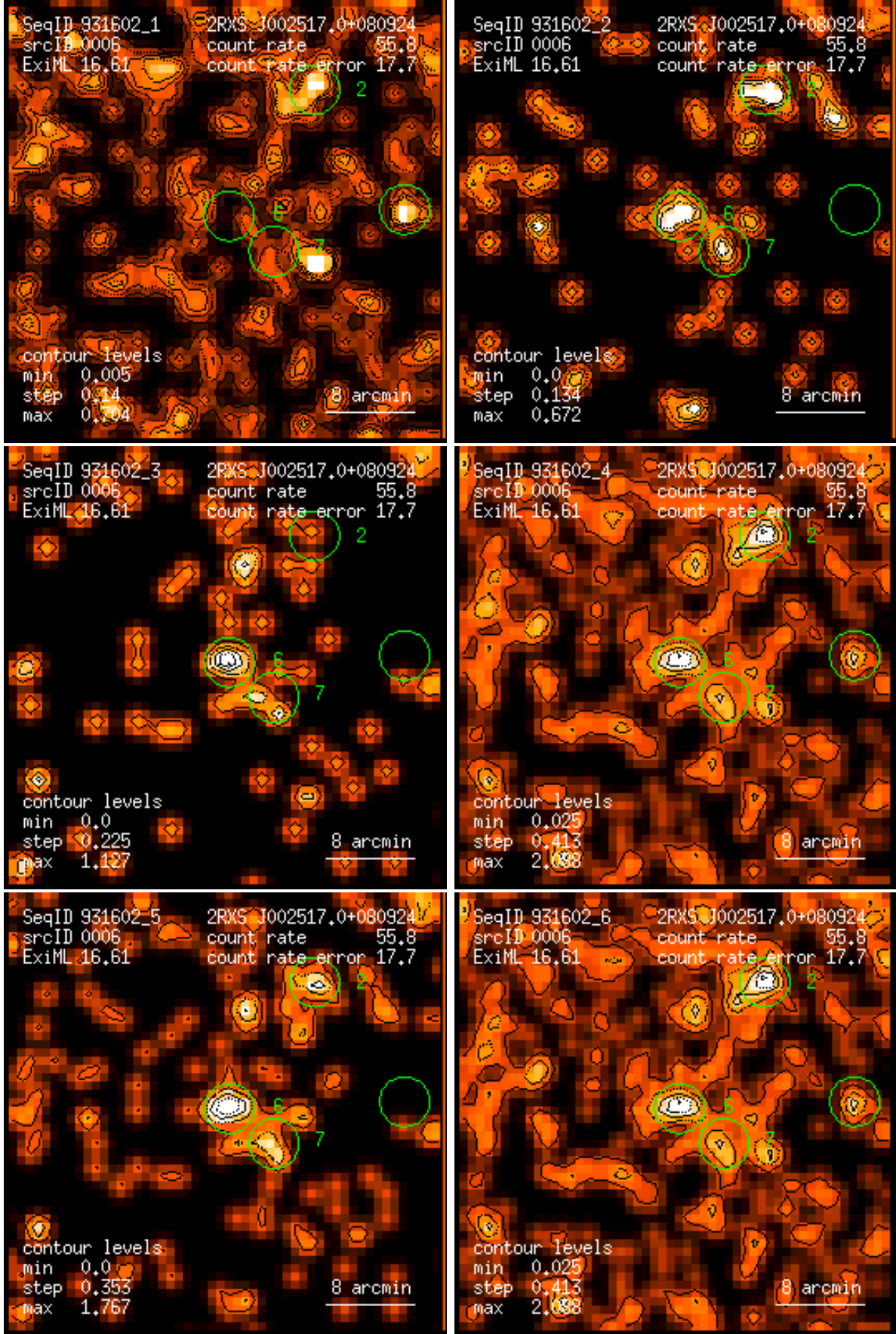
Figure 6: RASS 931602: detection 0006: band rate images, Gaussian filter: (1) PSPC channels 11 – 41, (2) 52 – 90, (3) 91 – 201, (4) 11 – 235, (5) 52 – 201, (6) 11 – 201. Broad band rates in counts/ks. Band rate contour levels in counts/ks/arcmin 2 .
