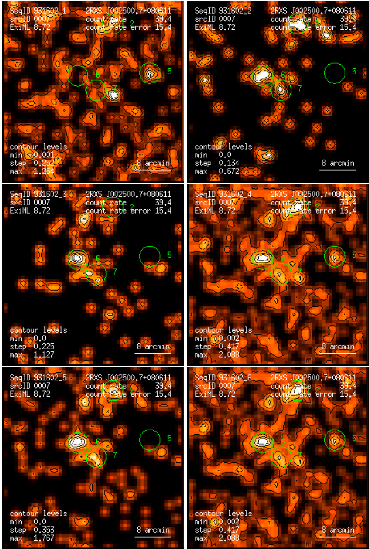
Figure 7: RASS 931602: detection 0007: band rate images, Gaussian filter: (1) PSPC channels 11 – 41, (2) 52 – 90, (3) 91 – 201, (4) 11 – 235, (5) 52 – 201, (6) 11 – 201. Broad band rates in counts/ks. Band rate contour levels in counts/ks/arcmin 2 .
