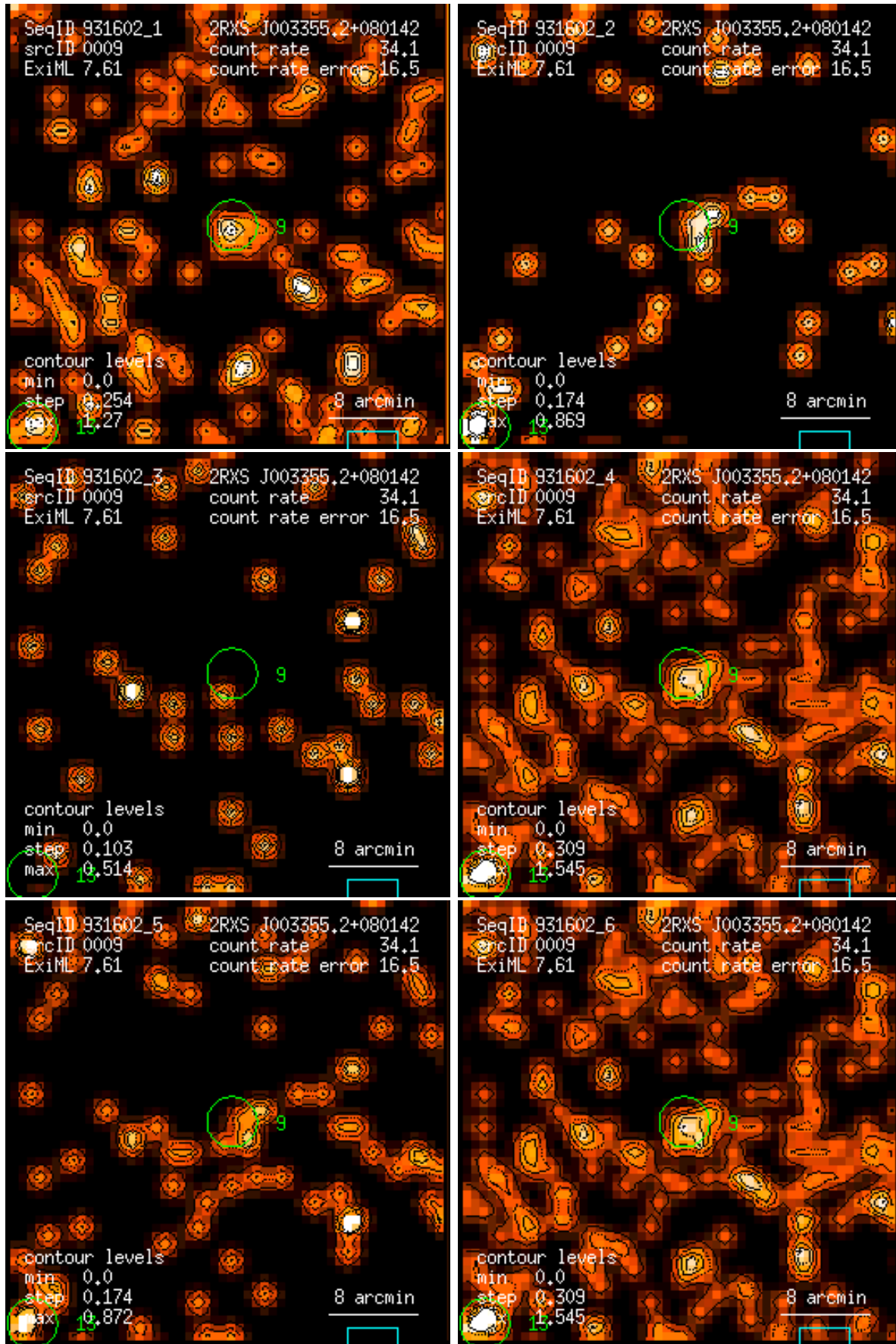
Figure 9: RASS 931602: detection 0009: band rate images, Gaussian filter: (1) PSPC channels 11 – 41, (2) 52 – 90, (3) 91 – 201, (4) 11 – 235, (5) 52 – 201, (6) 11 – 201. Broad band rates in counts/ks. Band rate contour levels in counts/ks/arcmin 2 .
