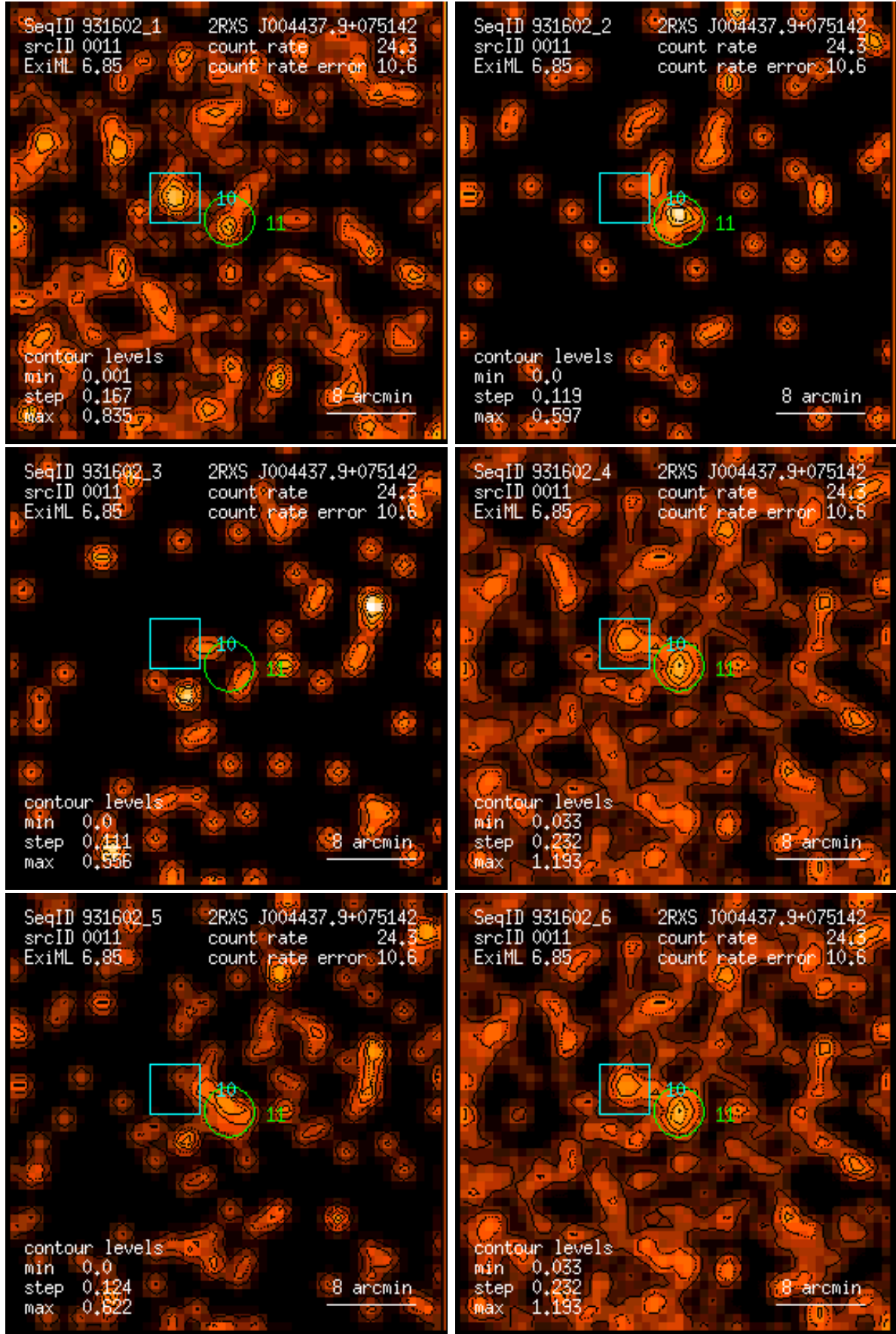
Figure 11: RASS 931602: detection 0011: band rate images, Gaussian filter: (1) PSPC channels 11 – 41, (2) 52 – 90, (3) 91 – 201, (4) 11 – 235, (5) 52 – 201, (6) 11 – 201. Broad band rates in counts/ks. Band rate contour levels in counts/ks/arcmin 2 .
