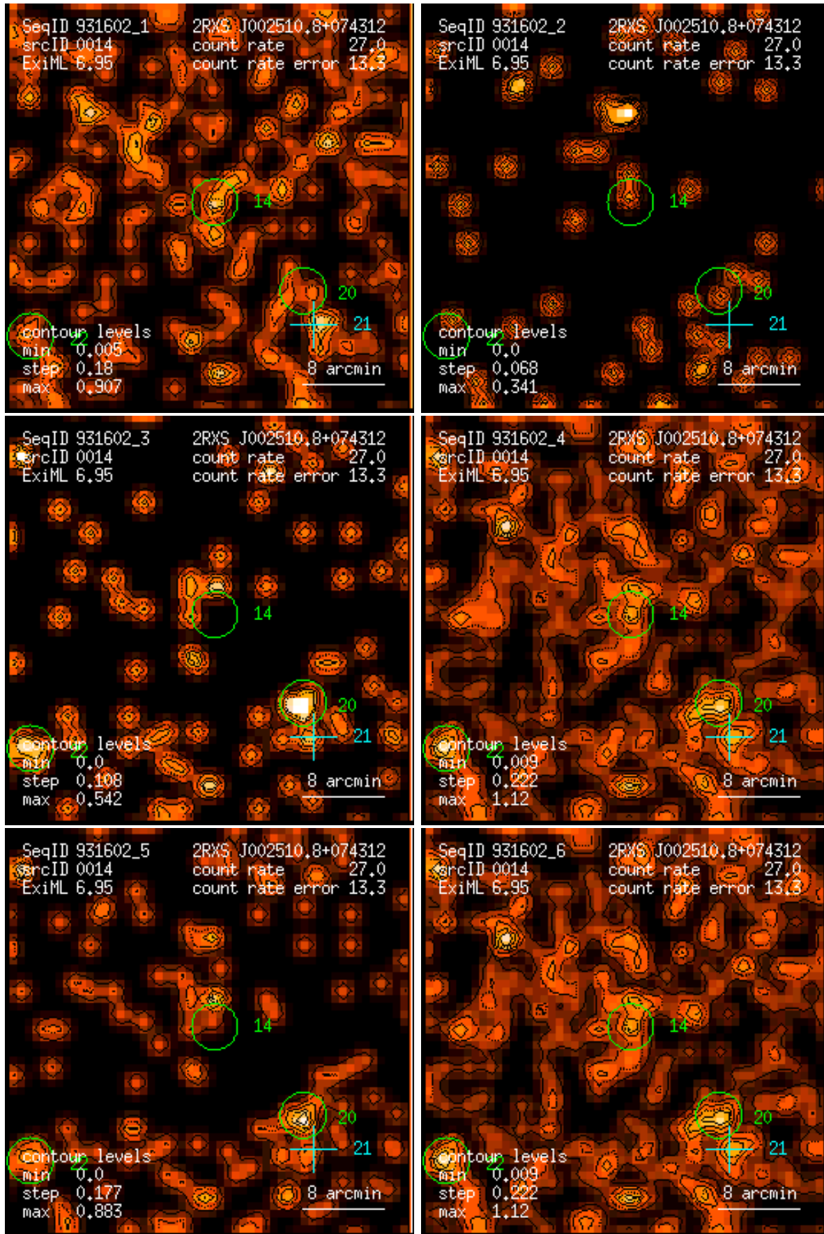
Figure 14: RASS 931602: detection 0014: band rate images, Gaussian filter: (1) PSPC channels 11 – 41, (2) 52 – 90, (3) 91 – 201, (4) 11 – 235, (5) 52 – 201, (6) 11 – 201. Broad band rates in counts/ks. Band rate contour levels in counts/ks/arcmin 2 .
