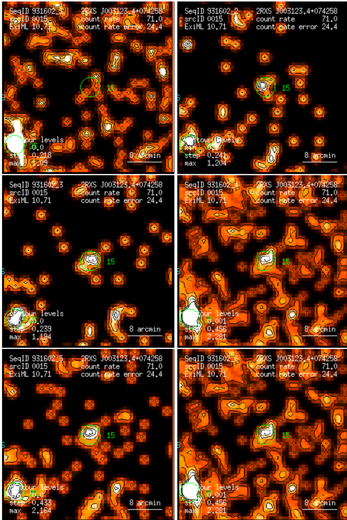
Figure 15: RASS 931602: detection 0015: band rate images, Gaussian filter: (1) PSPC channels 11 – 41, (2) 52 – 90, (3) 91 – 201, (4) 11 – 235, (5) 52 – 201, (6) 11 – 201. Broad band rates in counts/ks. Band rate contour levels in counts/ks/arcmin 2 .
