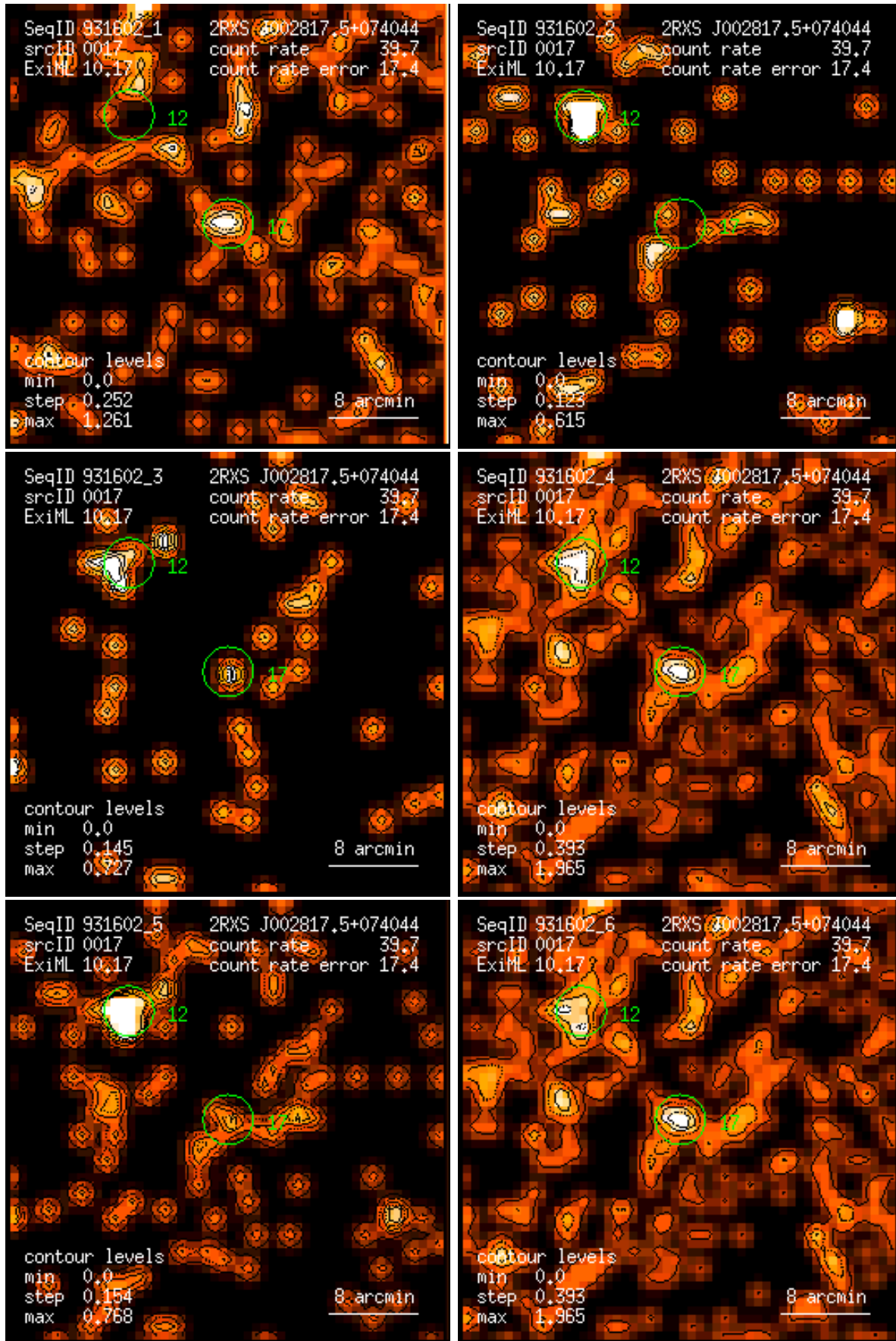
Figure 17: RASS 931602: detection 0017: band rate images, Gaussian filter: (1) PSPC channels 11 – 41, (2) 52 – 90, (3) 91 – 201, (4) 11 – 235, (5) 52 – 201, (6) 11 – 201. Broad band rates in counts/ks. Band rate contour levels in counts/ks/arcmin 2 .
