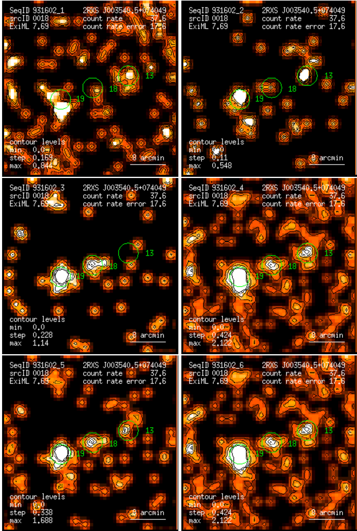
Figure 18: RASS 931602: detection 0018: band rate images, Gaussian filter: (1) PSPC channels 11 – 41, (2) 52 – 90, (3) 91 – 201, (4) 11 – 235, (5) 52 – 201, (6) 11 – 201. Broad band rates in counts/ks. Band rate contour levels in counts/ks/arcmin 2 .
