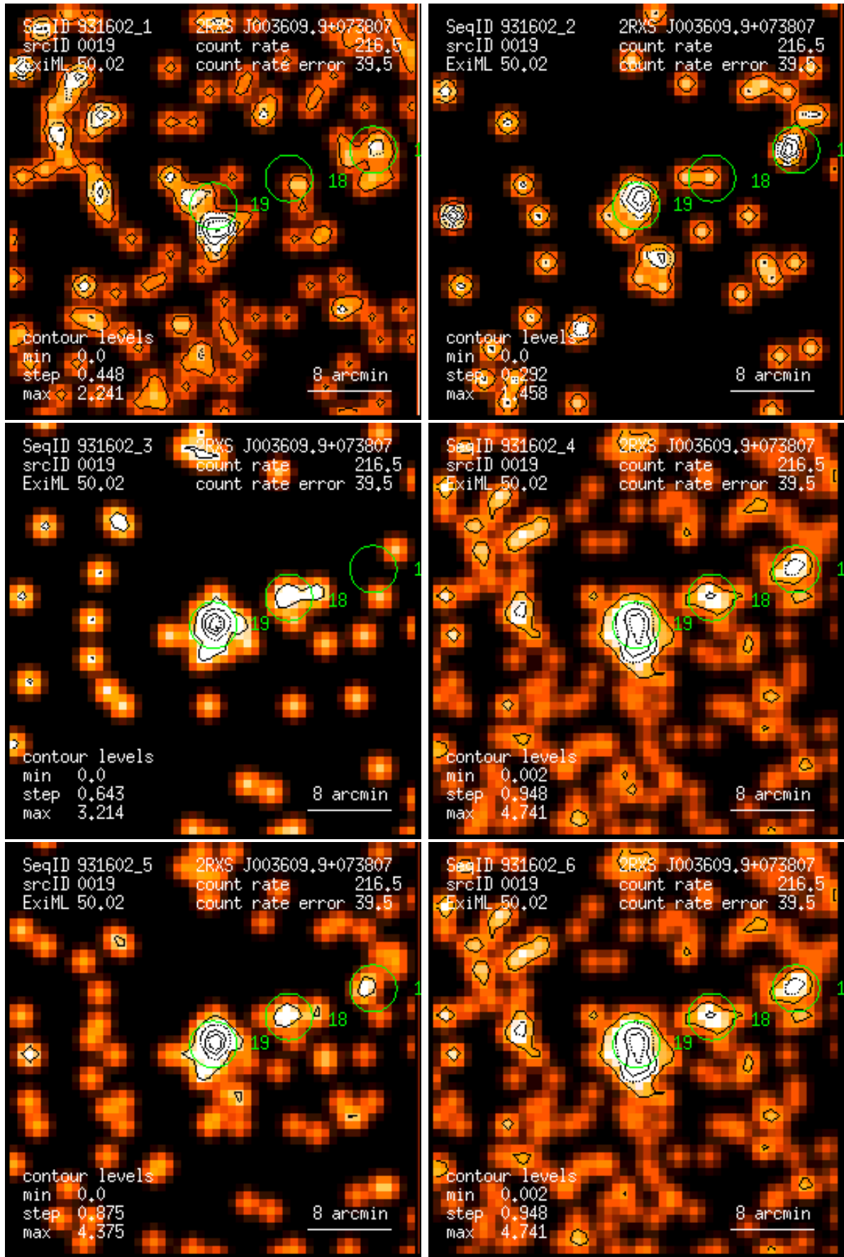
Figure 19: RASS 931602: detection 0019: band rate images, Gaussian filter: (1) PSPC channels 11 – 41, (2) 52 – 90, (3) 91 – 201, (4) 11 – 235, (5) 52 – 201, (6) 11 – 201. Broad band rates in counts/ks. Band rate contour levels in counts/ks/arcmin 2 .
