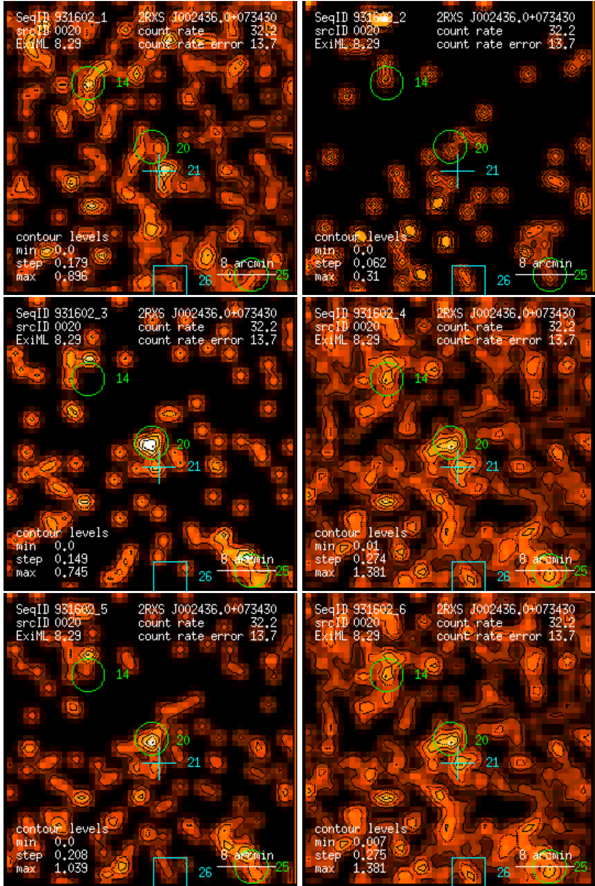
Figure 20: RASS 931602: detection 0020: band rate images, Gaussian filter: (1) PSPC channels 11 – 41, (2) 52 – 90, (3) 91 – 201, (4) 11 – 235, (5) 52 – 201, (6) 11 – 201. Broad band rates in counts/ks. Band rate contour levels in counts/ks/arcmin 2 .
