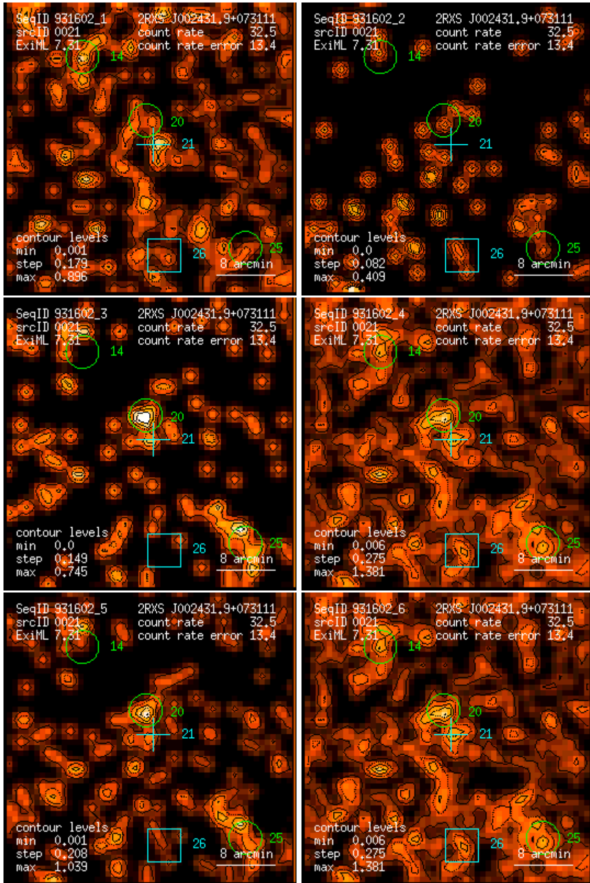
Figure 21: RASS 931602: detection 0021: band rate images, Gaussian filter: (1) PSPC channels 11 – 41, (2) 52 – 90, (3) 91 – 201, (4) 11 – 235, (5) 52 – 201, (6) 11 – 201. Broad band rates in counts/ks. Band rate contour levels in counts/ks/arcmin 2 .
