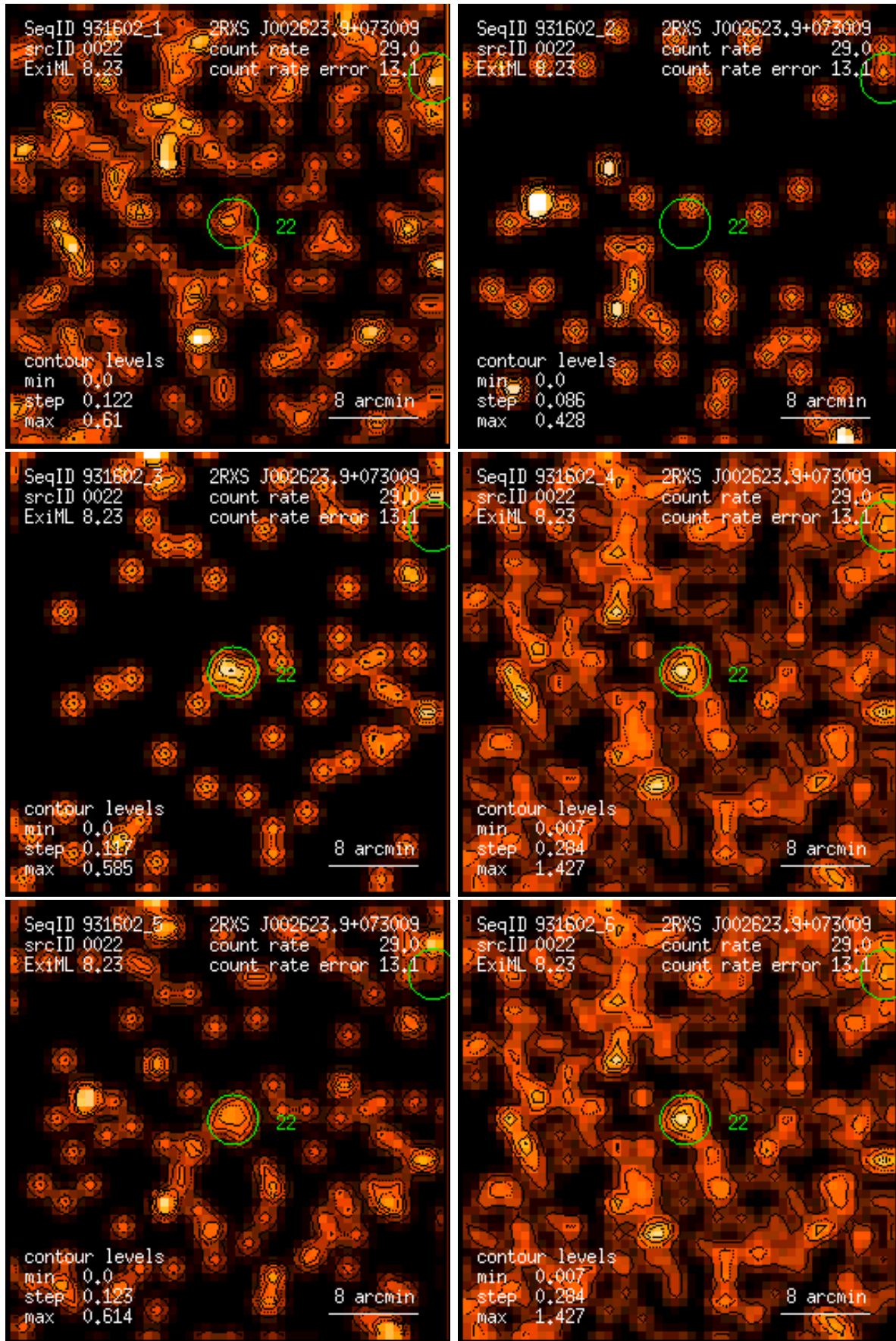
Figure 22: RASS 931602: detection 0022: band rate images, Gaussian filter: (1) PSPC channels 11 – 41, (2) 52 – 90, (3) 91 – 201, (4) 11 – 235, (5) 52 – 201, (6) 11 – 201. Broad band rates in counts/ks. Band rate contour levels in counts/ks/arcmin 2 .
