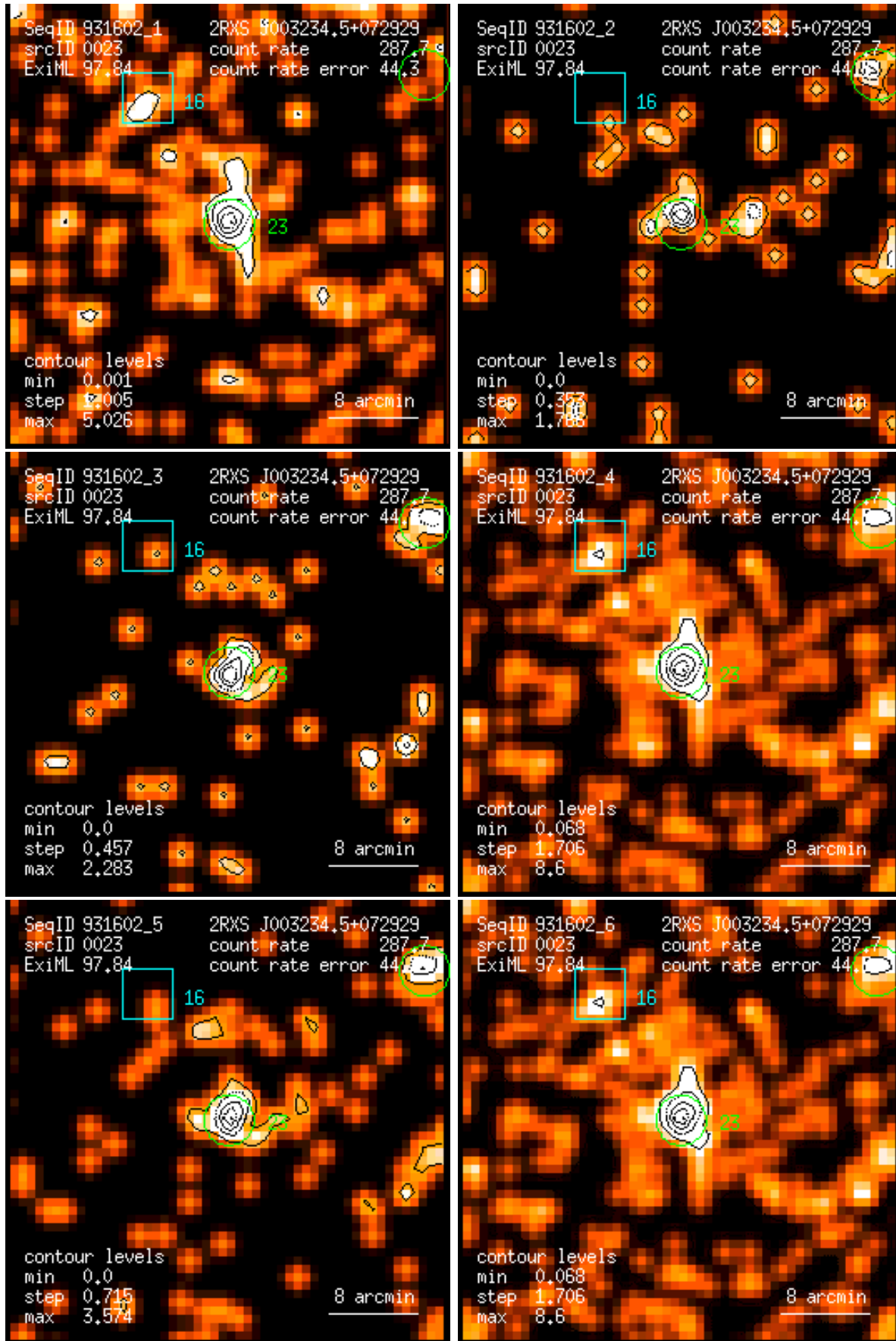
Figure 23: RASS 931602: detection 0023: band rate images, Gaussian filter: (1) PSPC channels 11 – 41, (2) 52 – 90, (3) 91 – 201, (4) 11 – 235, (5) 52 – 201, (6) 11 – 201. Broad band rates in counts/ks. Band rate contour levels in counts/ks/arcmin 2 .
