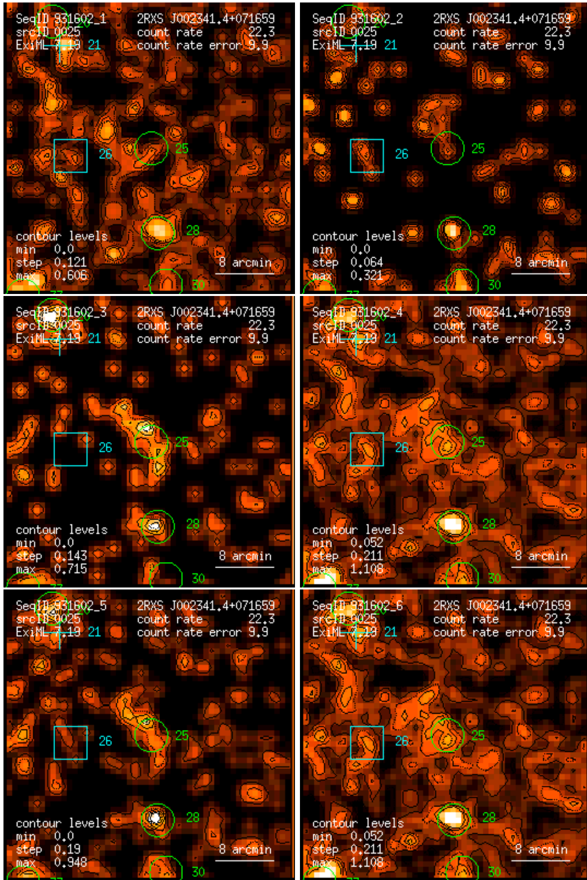
Figure 25: RASS 931602: detection 0025: band rate images, Gaussian filter: (1) PSPC channels 11 – 41, (2) 52 – 90, (3) 91 – 201, (4) 11 – 235, (5) 52 – 201, (6) 11 – 201. Broad band rates in counts/ks. Band rate contour levels in counts/ks/arcmin 2 .
