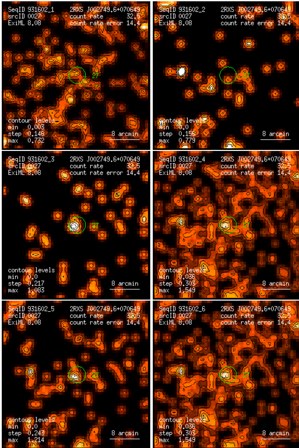
Figure 27: RASS 931602: detection 0027: band rate images, Gaussian filter: (1) PSPC channels 11 – 41, (2) 52 – 90, (3) 91 – 201, (4) 11 – 235, (5) 52 – 201, (6) 11 – 201. Broad band rates in counts/ks. Band rate contour levels in counts/ks/arcmin 2 .
