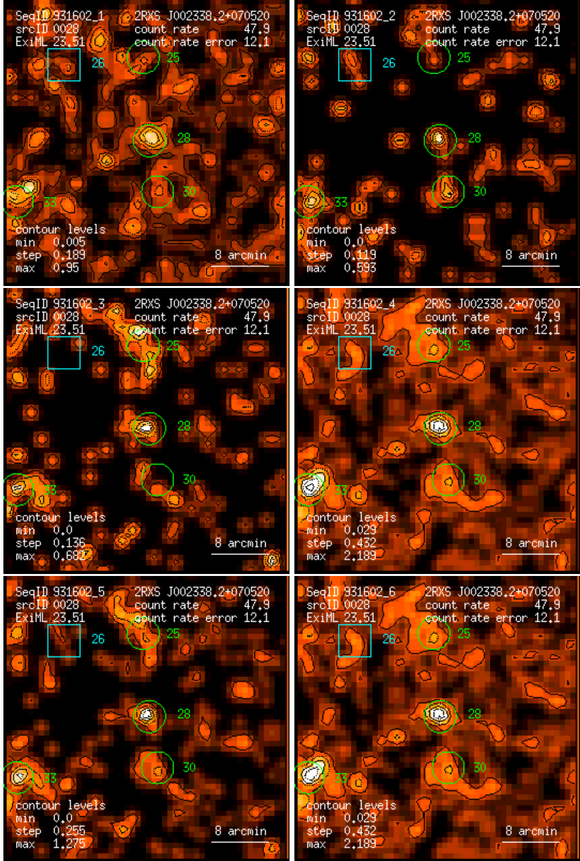
Figure 28: RASS 931602: detection 0028: band rate images, Gaussian filter: (1) PSPC channels 11 – 41, (2) 52 – 90, (3) 91 – 201, (4) 11 – 235, (5) 52 – 201, (6) 11 – 201. Broad band rates in counts/ks. Band rate contour levels in counts/ks/arcmin 2 .
