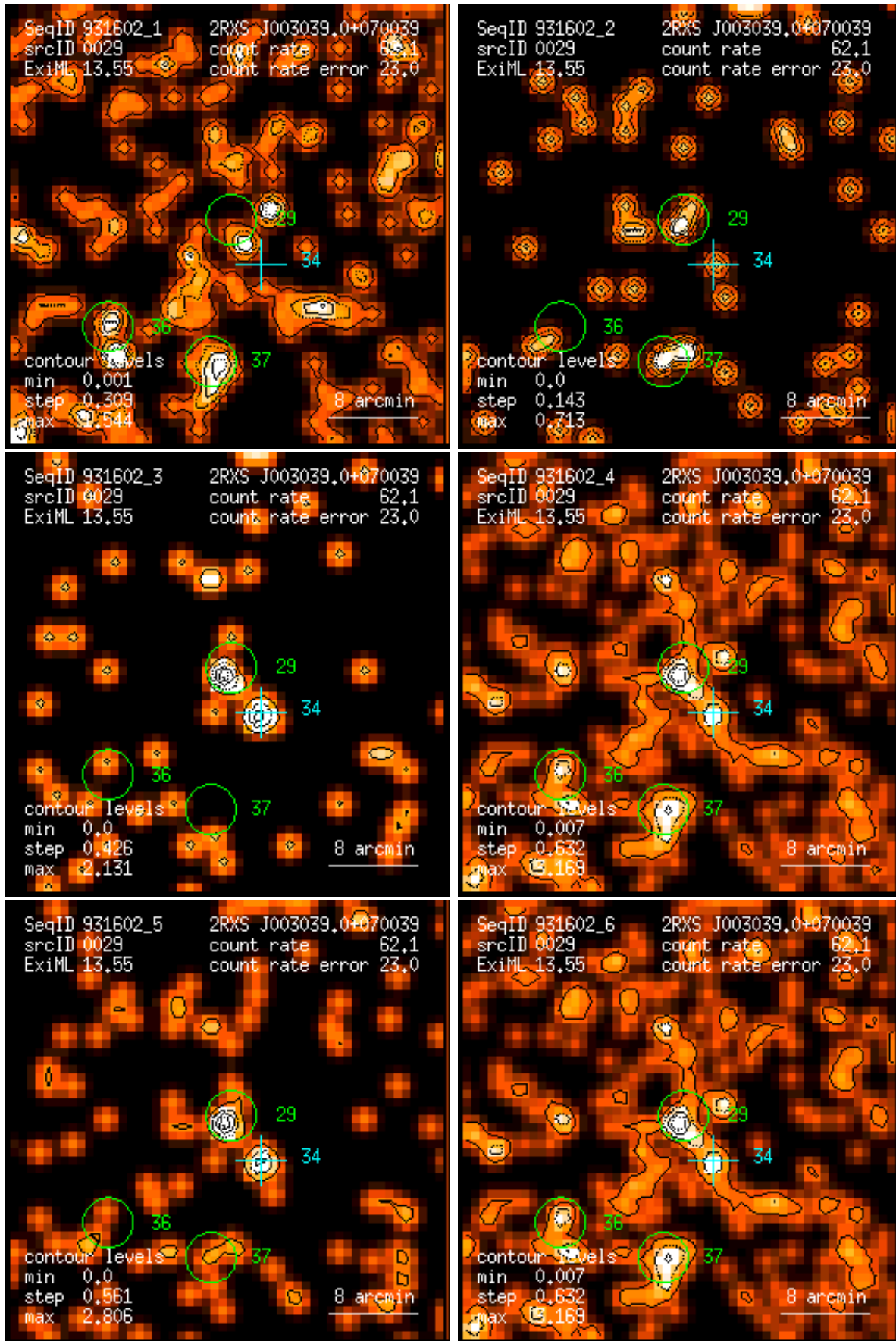
Figure 29: RASS 931602: detection 0029: band rate images, Gaussian filter: (1) PSPC channels 11 – 41, (2) 52 – 90, (3) 91 – 201, (4) 11 – 235, (5) 52 – 201, (6) 11 – 201. Broad band rates in counts/ks. Band rate contour levels in counts/ks/arcmin 2 .
