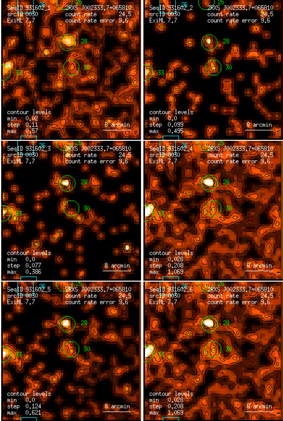
Figure 30: RASS 931602: detection 0030: band rate images, Gaussian filter: (1) PSPC channels 11 – 41, (2) 52 – 90, (3) 91 – 201, (4) 11 – 235, (5) 52 – 201, (6) 11 – 201. Broad band rates in counts/ks. Band rate contour levels in counts/ks/arcmin 2 .
