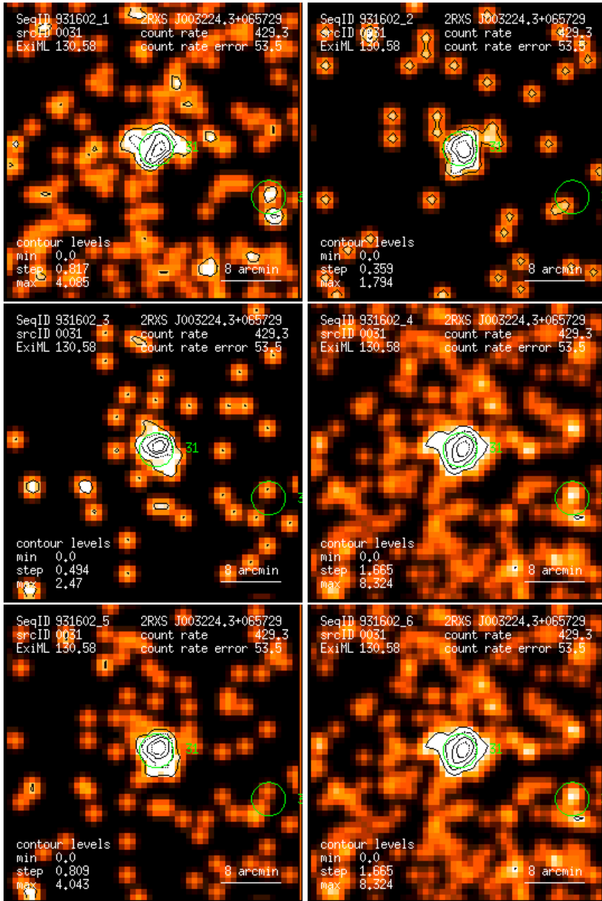
Figure 31: RASS 931602: detection 0031: band rate images, Gaussian filter: (1) PSPC channels 11 – 41, (2) 52 – 90, (3) 91 – 201, (4) 11 – 235, (5) 52 – 201, (6) 11 – 201. Broad band rates in counts/ks. Band rate contour levels in counts/ks/arcmin 2 .
