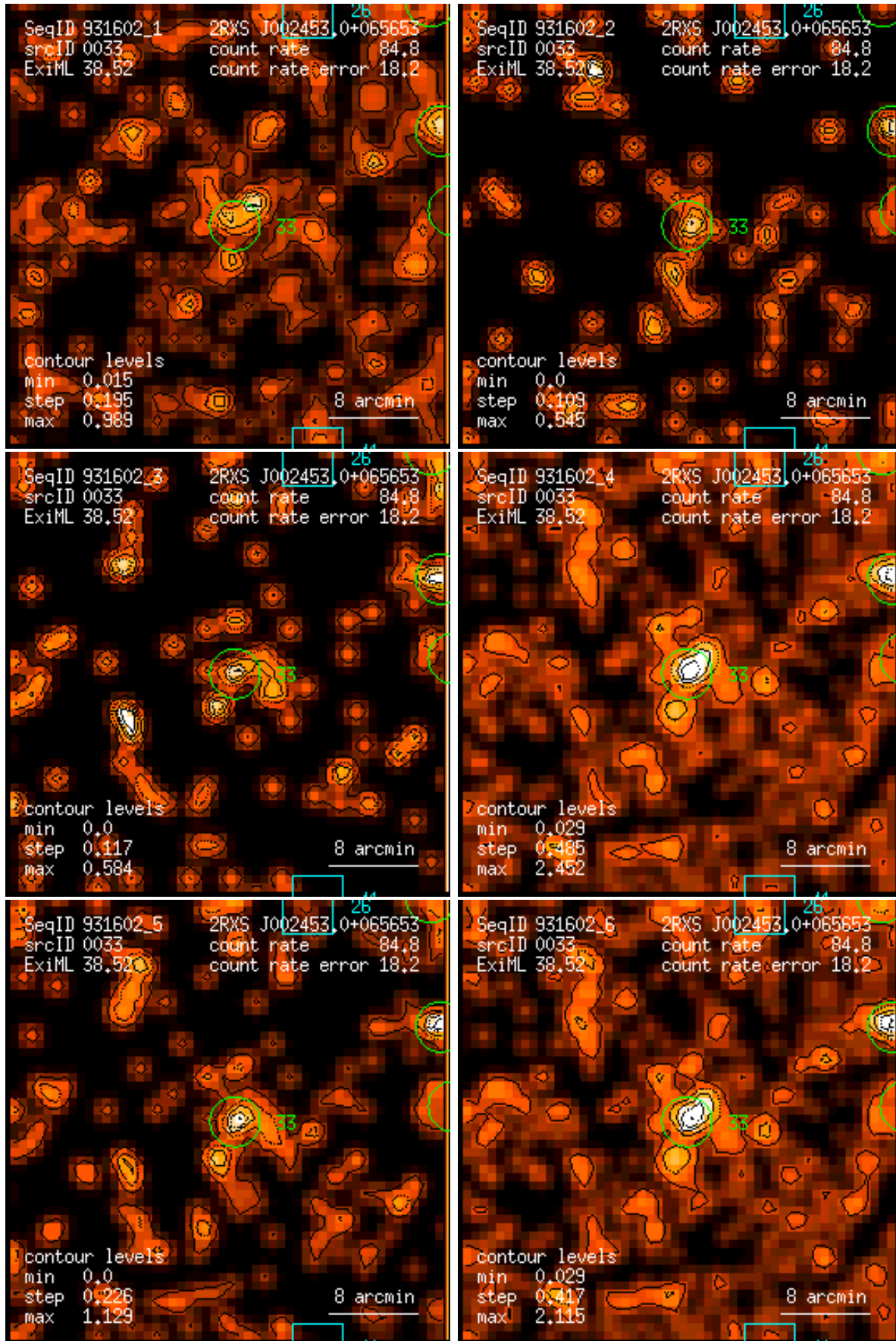
Figure 33: RASS 931602: detection 0033: band rate images, Gaussian filter: (1) PSPC channels 11 – 41, (2) 52 – 90, (3) 91 – 201, (4) 11 – 235, (5) 52 – 201, (6) 11 – 201. Broad band rates in counts/ks. Band rate contour levels in counts/ks/arcmin 2 .
