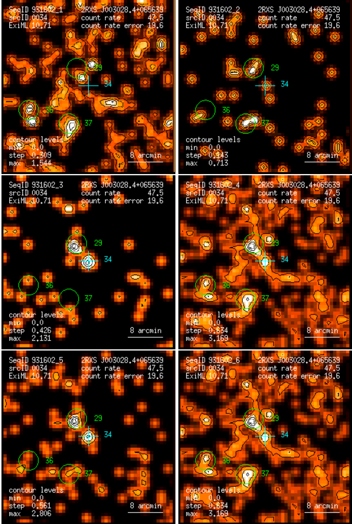
Figure 34: RASS 931602: detection 0034: band rate images, Gaussian filter: (1) PSPC channels 11 – 41, (2) 52 – 90, (3) 91 – 201, (4) 11 – 235, (5) 52 – 201, (6) 11 – 201. Broad band rates in counts/ks. Band rate contour levels in counts/ks/arcmin 2 .
