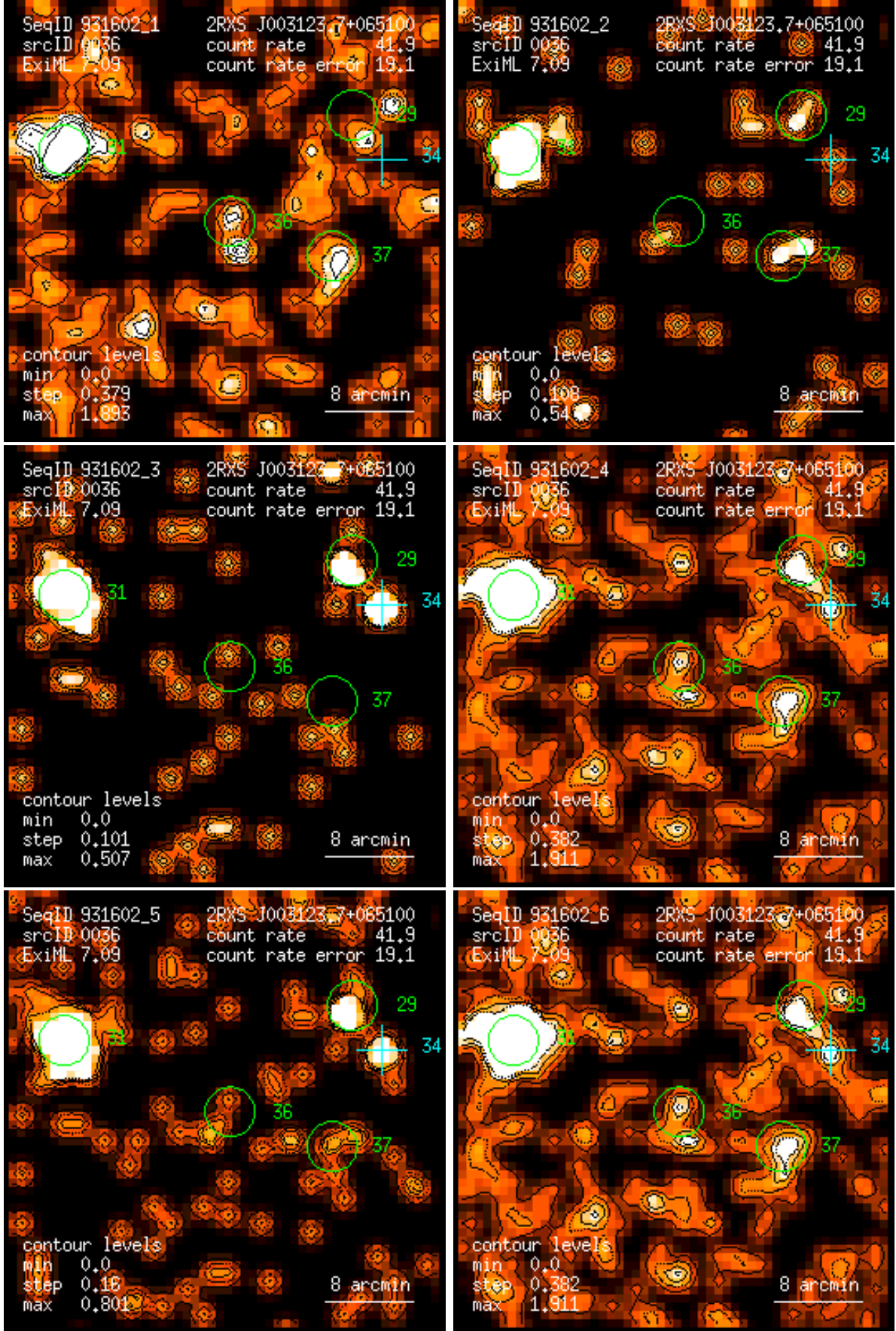
Figure 36: RASS 931602: detection 0036: band rate images, Gaussian filter: (1) PSPC channels 11 – 41, (2) 52 – 90, (3) 91 – 201, (4) 11 – 235, (5) 52 – 201, (6) 11 – 201. Broad band rates in counts/ks. Band rate contour levels in counts/ks/arcmin 2 .
