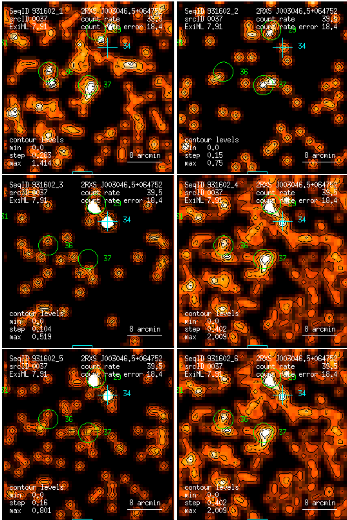
Figure 37: RASS 931602: detection 0037: band rate images, Gaussian filter: (1) PSPC channels 11 – 41, (2) 52 – 90, (3) 91 – 201, (4) 11 – 235, (5) 52 – 201, (6) 11 – 201. Broad band rates in counts/ks. Band rate contour levels in counts/ks/arcmin 2 .
