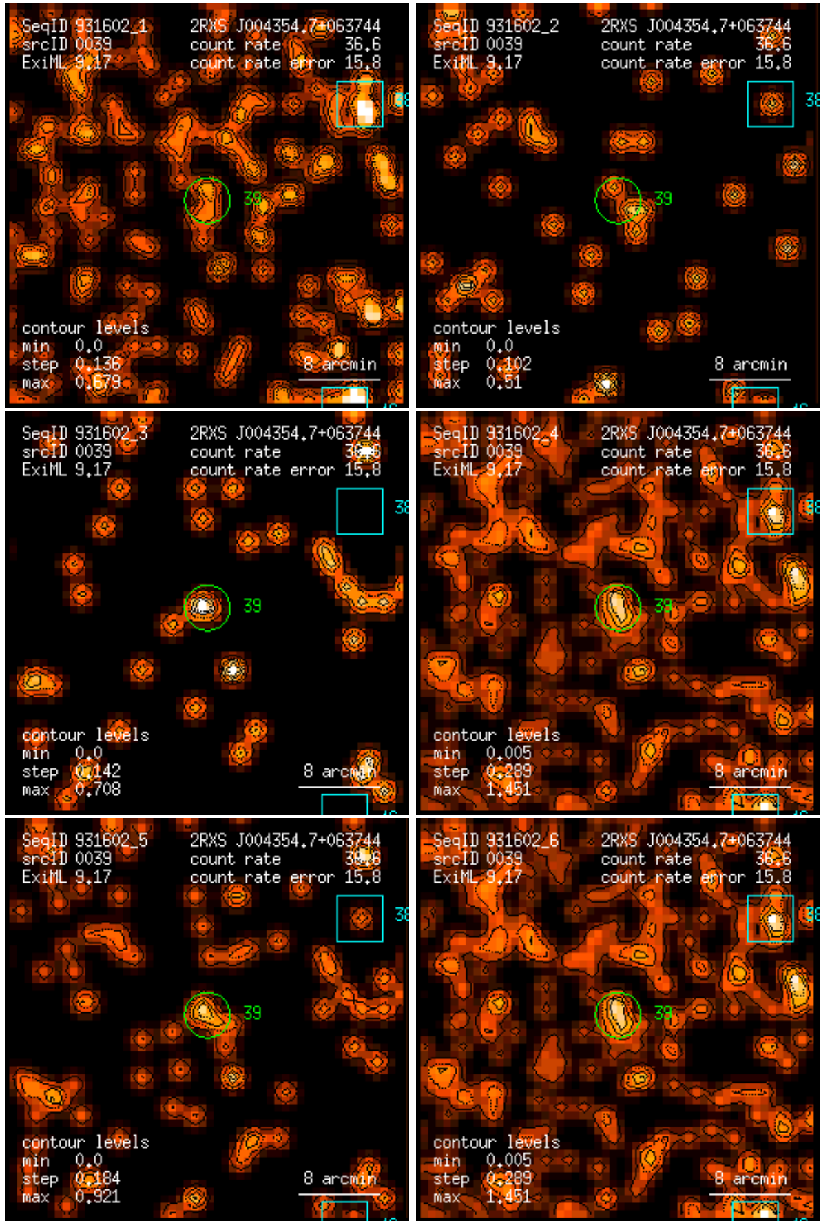
Figure 39: RASS 931602: detection 0039: band rate images, Gaussian filter: (1) PSPC channels 11 – 41, (2) 52 – 90, (3) 91 – 201, (4) 11 – 235, (5) 52 – 201, (6) 11 – 201. Broad band rates in counts/ks. Band rate contour levels in counts/ks/arcmin 2 .
