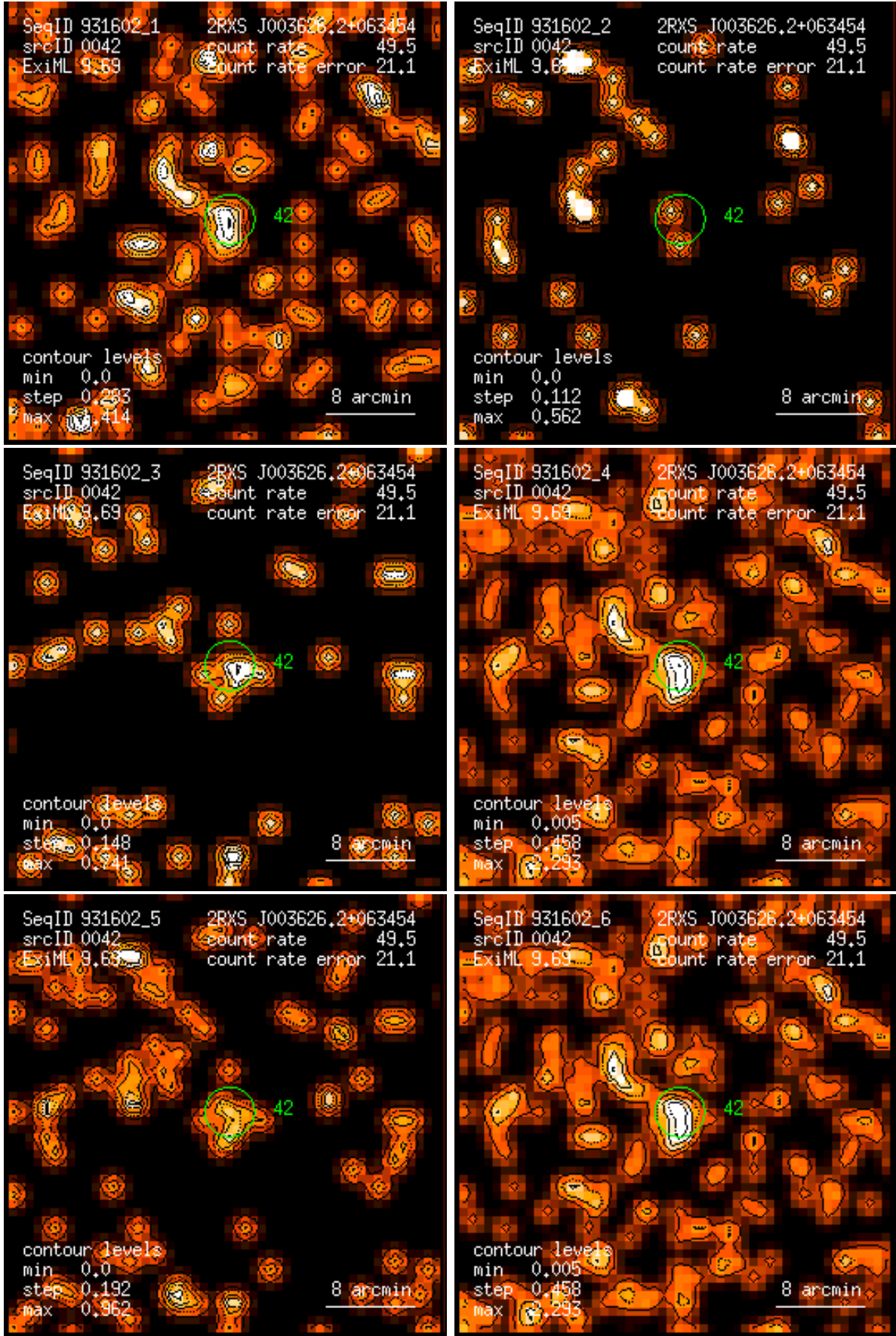
Figure 42: RASS 931602: detection 0042: band rate images, Gaussian filter: (1) PSPC channels 11 – 41, (2) 52 – 90, (3) 91 – 201, (4) 11 – 235, (5) 52 – 201, (6) 11 – 201. Broad band rates in counts/ks. Band rate contour levels in counts/ks/arcmin 2 .
