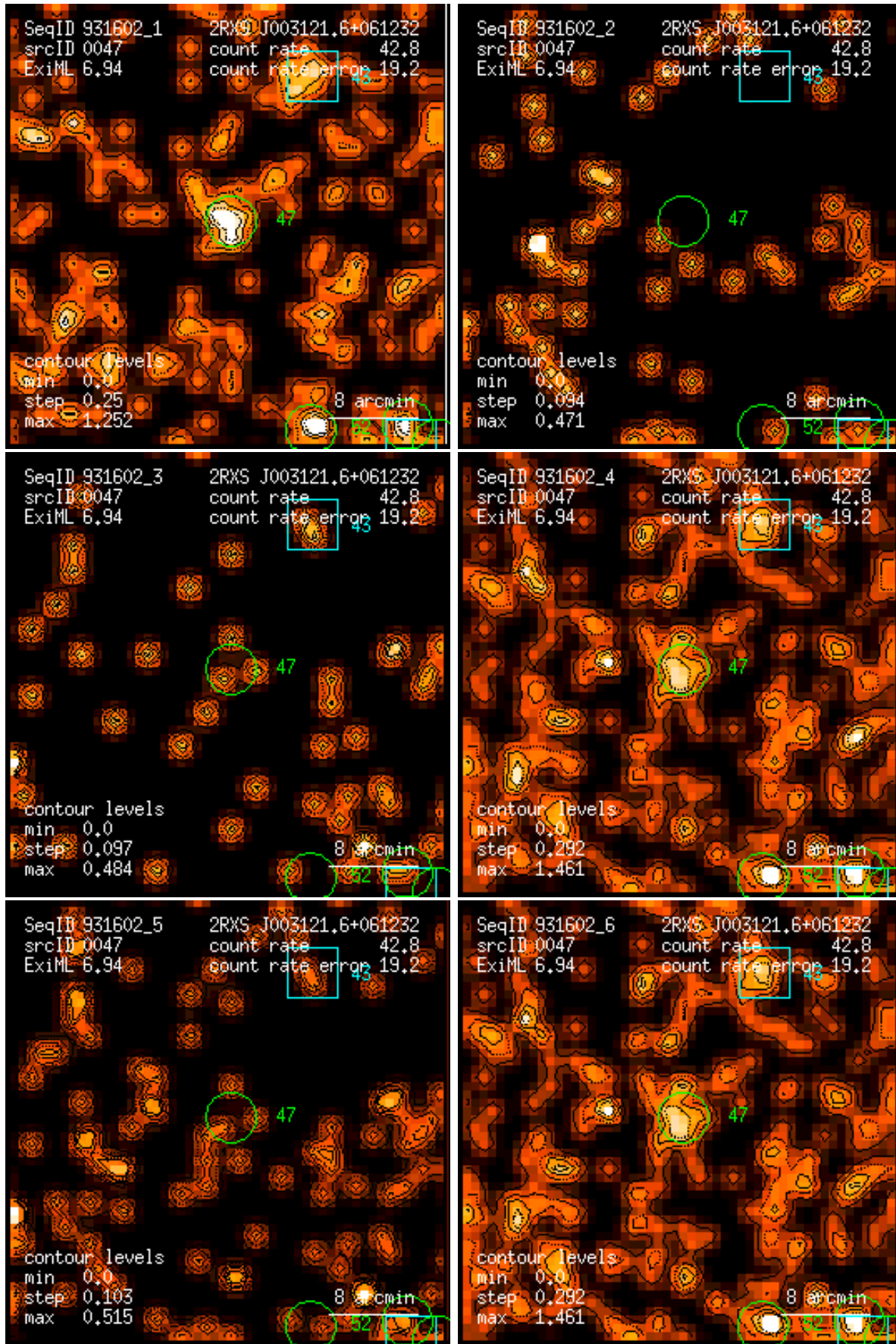
Figure 47: RASS 931602: detection 0047: band rate images, Gaussian filter: (1) PSPC channels 11 – 41, (2) 52 – 90, (3) 91 – 201, (4) 11 – 235, (5) 52 – 201, (6) 11 – 201. Broad band rates in counts/ks. Band rate contour levels in counts/ks/arcmin 2 .
