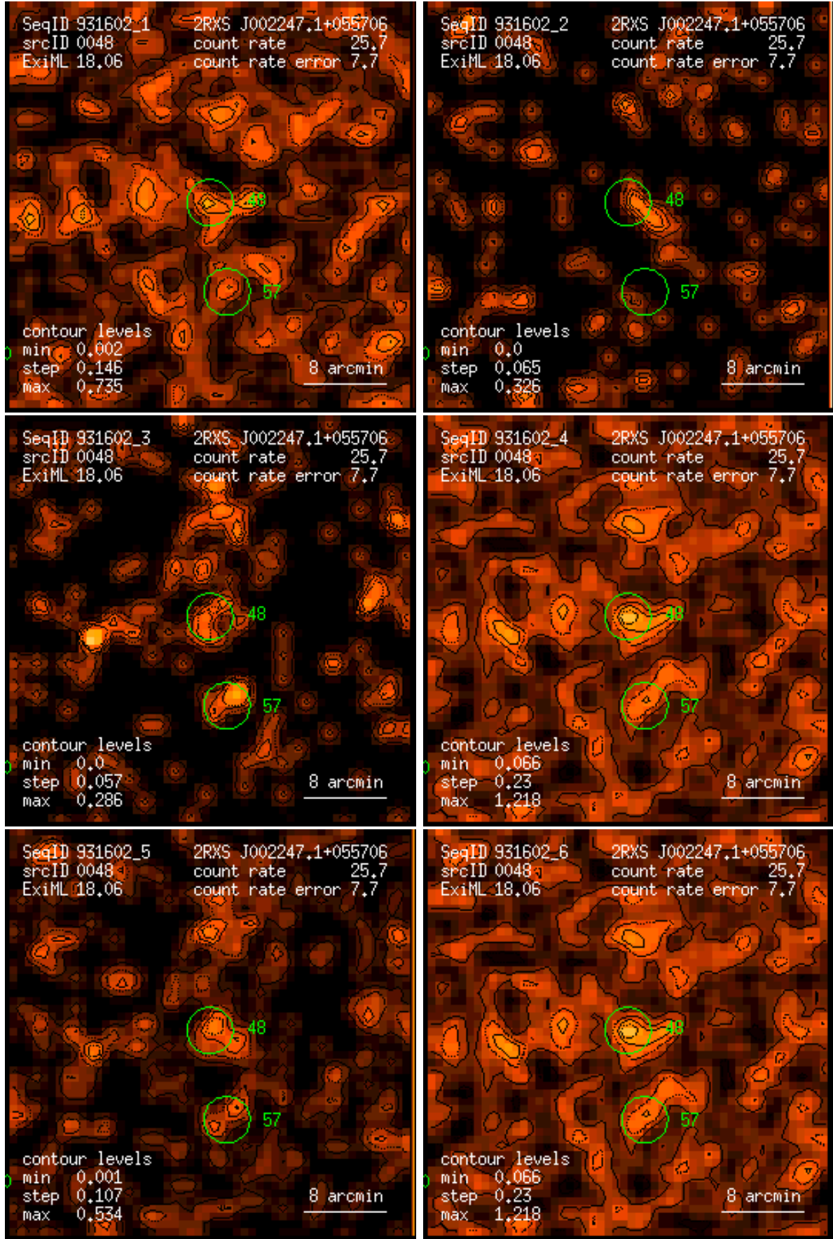
Figure 48: RASS 931602: detection 0048: band rate images, Gaussian filter: (1) PSPC channels 11 – 41, (2) 52 – 90, (3) 91 – 201, (4) 11 – 235, (5) 52 – 201, (6) 11 – 201. Broad band rates in counts/ks. Band rate contour levels in counts/ks/arcmin 2 .
