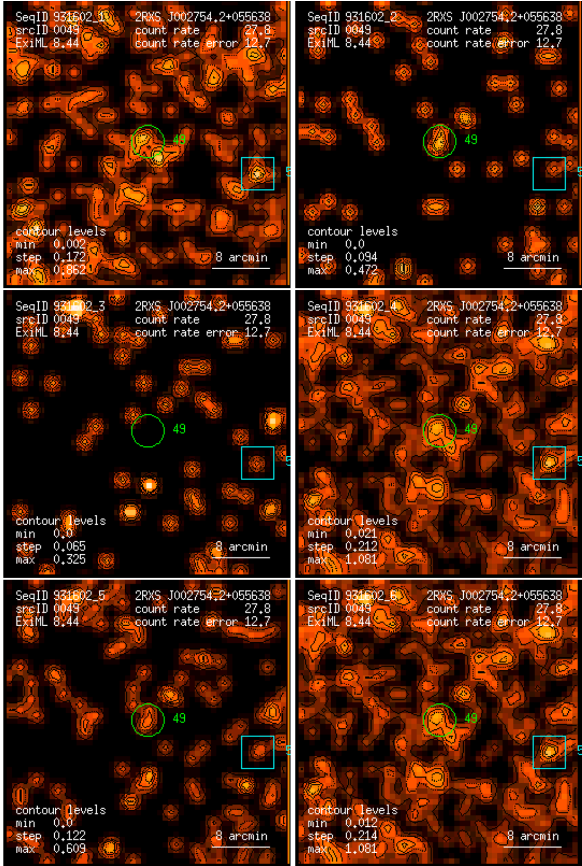
Figure 49: RASS 931602: detection 0049: band rate images, Gaussian filter: (1) PSPC channels 11 – 41, (2) 52 – 90, (3) 91 – 201, (4) 11 – 235, (5) 52 – 201, (6) 11 – 201. Broad band rates in counts/ks. Band rate contour levels in counts/ks/arcmin 2 .
