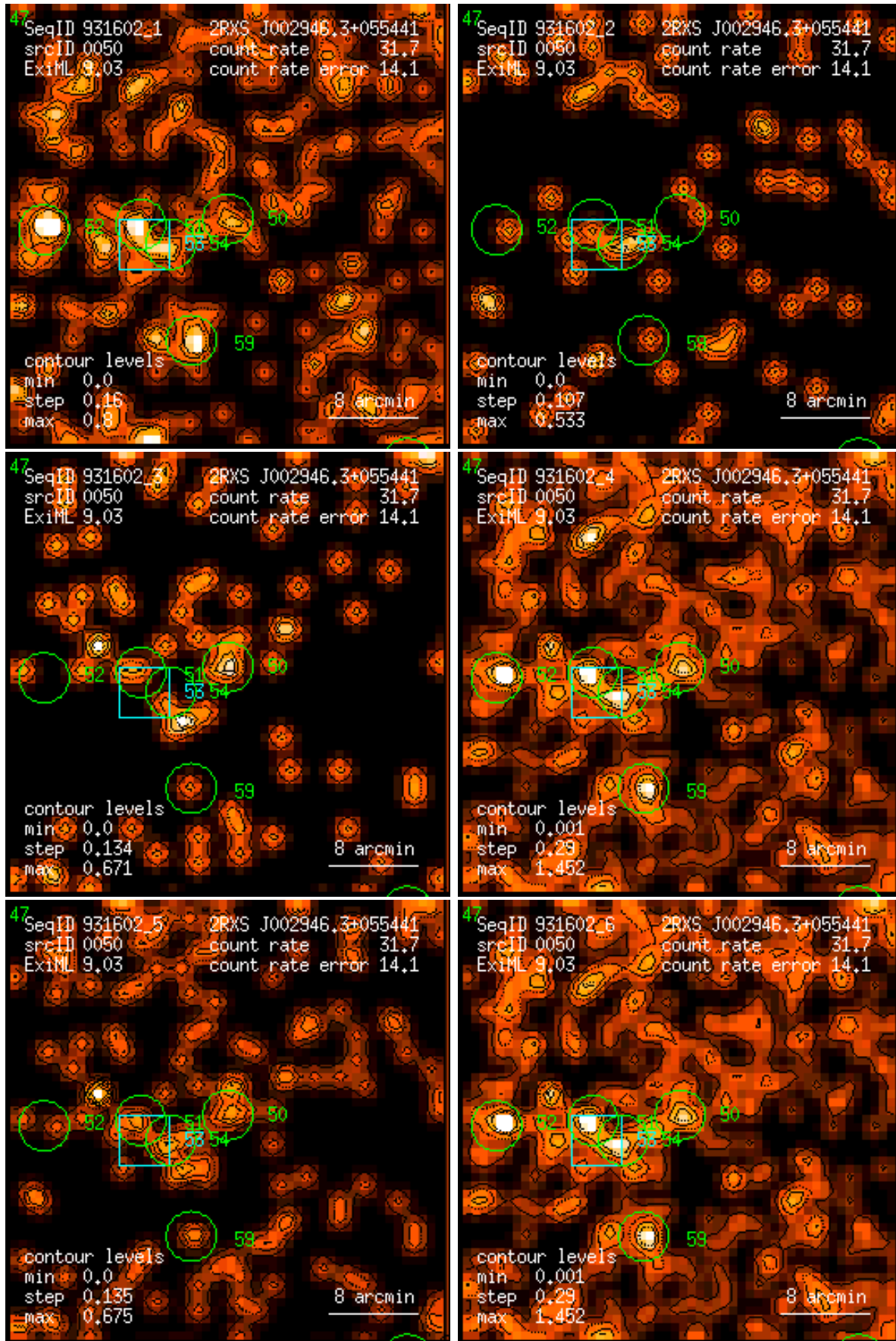
Figure 50: RASS 931602: detection 0050: band rate images, Gaussian filter: (1) PSPC channels 11 – 41, (2) 52 – 90, (3) 91 – 201, (4) 11 – 235, (5) 52 – 201, (6) 11 – 201. Broad band rates in counts/ks. Band rate contour levels in counts/ks/arcmin 2 .
