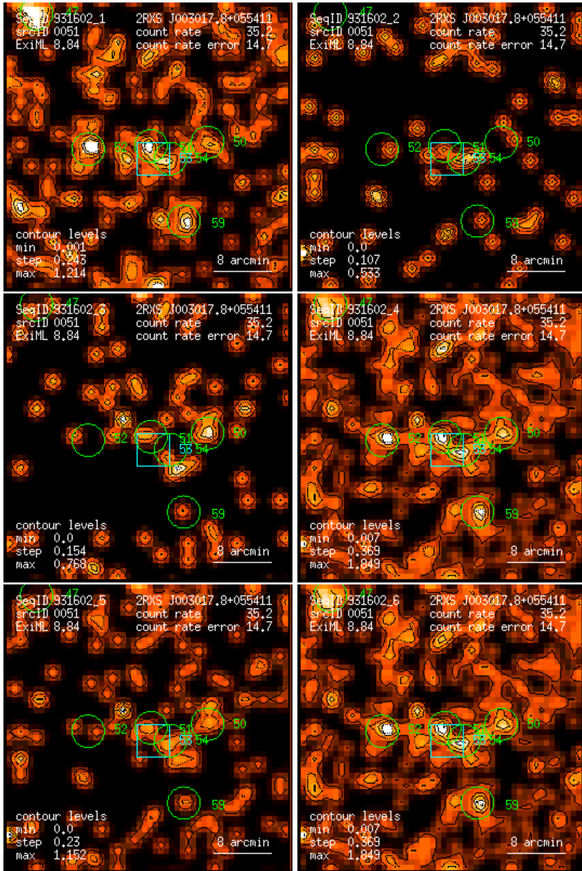
Figure 51: RASS 931602: detection 0051: band rate images, Gaussian filter: (1) PSPC channels 11 – 41, (2) 52 – 90, (3) 91 – 201, (4) 11 – 235, (5) 52 – 201, (6) 11 – 201. Broad band rates in counts/ks. Band rate contour levels in counts/ks/arcmin 2 .
