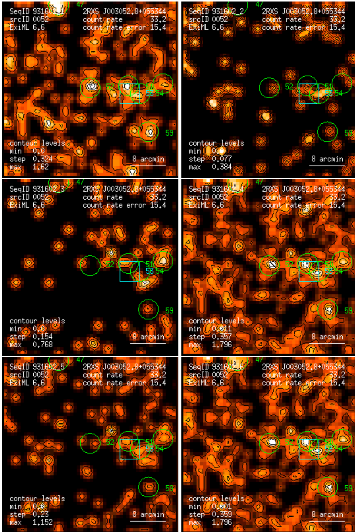
Figure 52: RASS 931602: detection 0052: band rate images, Gaussian filter: (1) PSPC channels 11 – 41, (2) 52 – 90, (3) 91 – 201, (4) 11 – 235, (5) 52 – 201, (6) 11 – 201. Broad band rates in counts/ks. Band rate contour levels in counts/ks/arcmin 2 .
