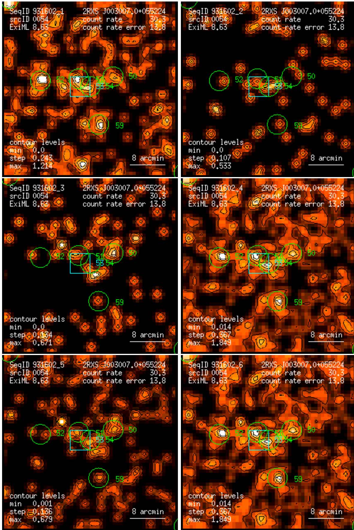
Figure 54: RASS 931602: detection 0054: band rate images, Gaussian filter: (1) PSPC channels 11 – 41, (2) 52 – 90, (3) 91 – 201, (4) 11 – 235, (5) 52 – 201, (6) 11 – 201. Broad band rates in counts/ks. Band rate contour levels in counts/ks/arcmin 2 .
