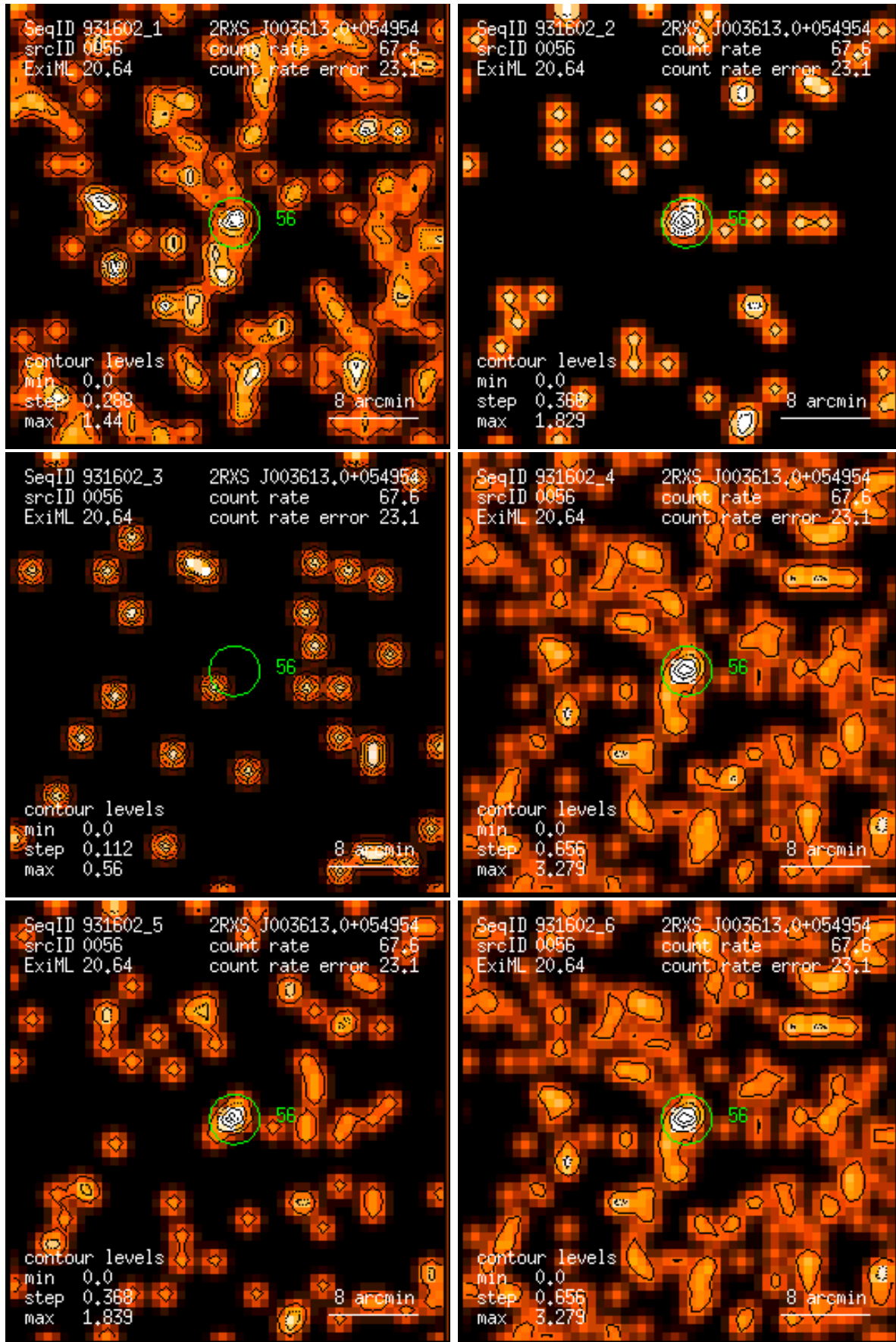
Figure 56: RASS 931602: detection 0056: band rate images, Gaussian filter: (1) PSPC channels 11 – 41, (2) 52 – 90, (3) 91 – 201, (4) 11 – 235, (5) 52 – 201, (6) 11 – 201. Broad band rates in counts/ks. Band rate contour levels in counts/ks/arcmin 2 .
