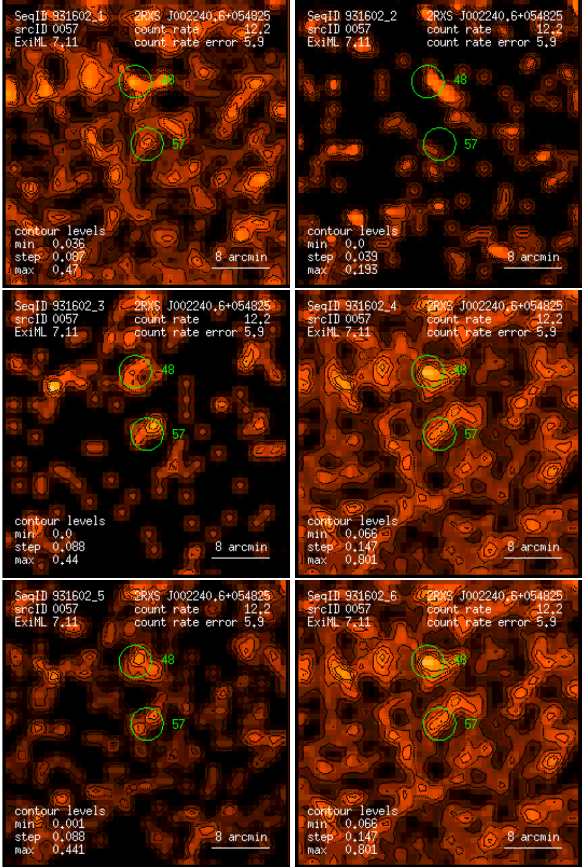
Figure 57: RASS 931602: detection 0057: band rate images, Gaussian filter: (1) PSPC channels 11 – 41, (2) 52 – 90, (3) 91 – 201, (4) 11 – 235, (5) 52 – 201, (6) 11 – 201. Broad band rates in counts/ks. Band rate contour levels in counts/ks/arcmin 2 .
