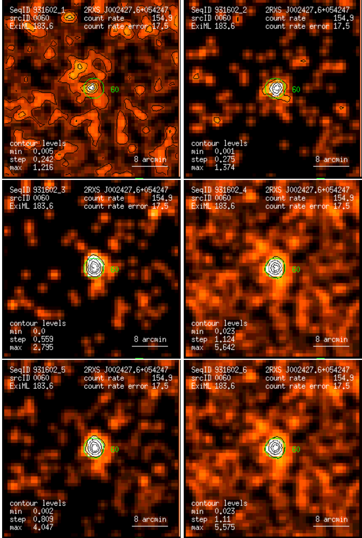
Figure 60: RASS 931602: detection 0060: band rate images, Gaussian filter: (1) PSPC channels 11 – 41, (2) 52 – 90, (3) 91 – 201, (4) 11 – 235, (5) 52 – 201, (6) 11 – 201. Broad band rates in counts/ks. Band rate contour levels in counts/ks/arcmin 2 .
